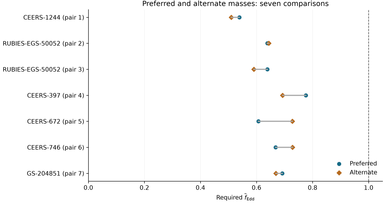
Figure 6: Preferred (circles) and alternate (diamonds) point requirements for seven measurement pairs across six primary objects. Pair numbers follow the released alternate-measurement table, which supplies stable measurement IDs; RUBIES-EGS-50052 (CEERS-2782) has two alternatives. All pairs remain below the reference threshold.
