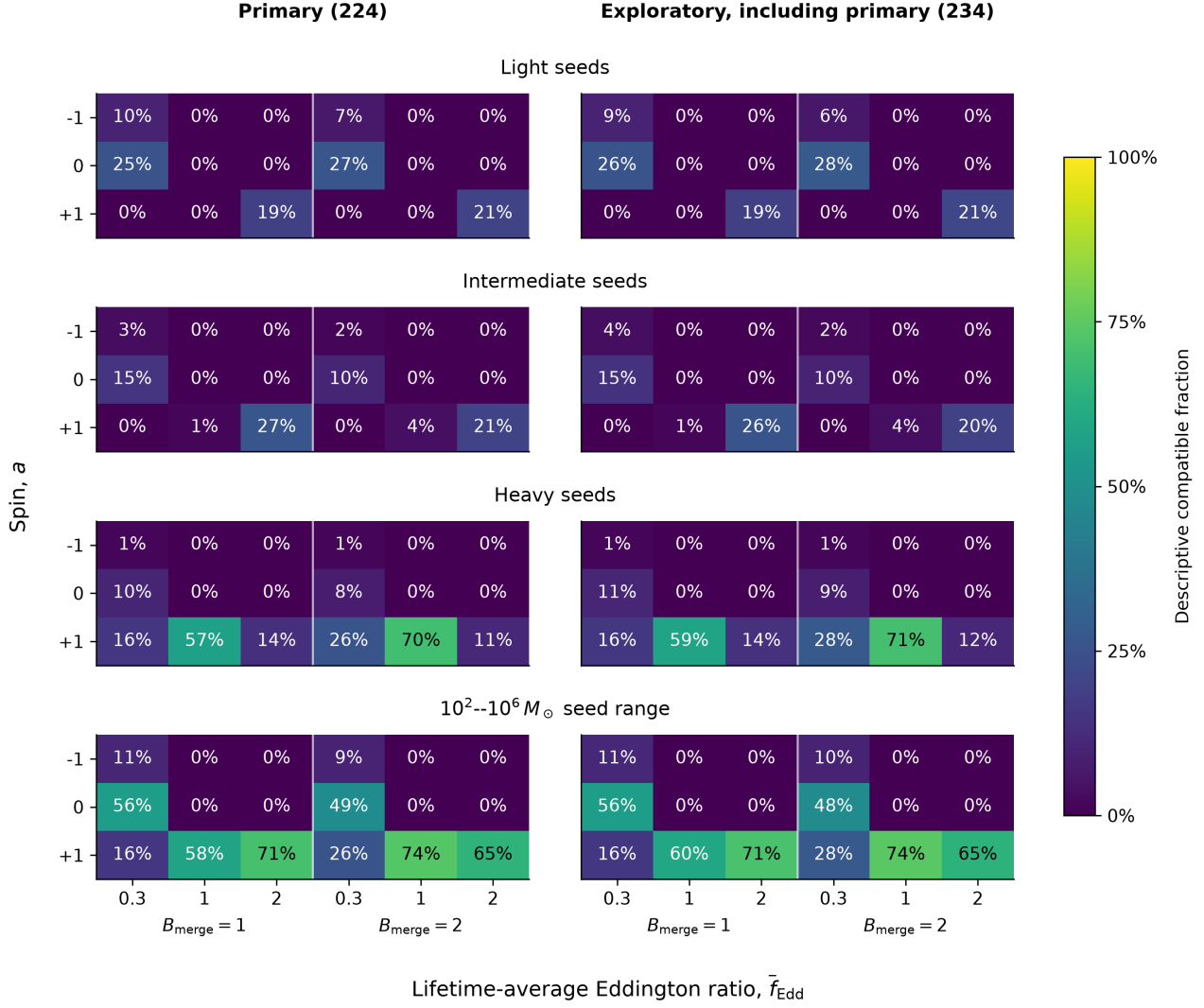
Figure 5: Constant-state compatibility fractions in the primary sample (left) and the inclusive exploratory sample (right). These samples are nested. Each column specifies merger multiplier B and fixed luminosity ratio f ; rows specify ideal spin-dependent efficiency, with the supercritical prescription in Appendix C. Seed intervals overlap and carry no probability weights. The broad mass interval has no formation-channel interpretation.
