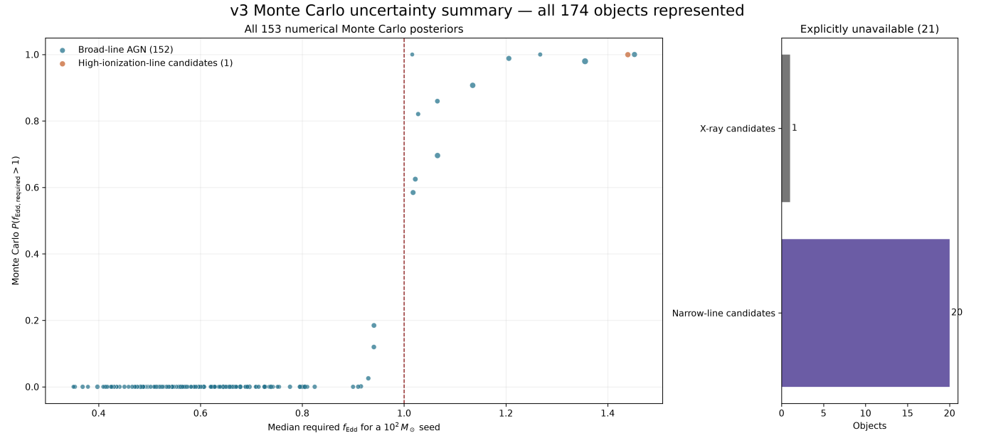
Figure 4. Monte Carlo pressure summary for all 153 numerical objects, with an explicit accounting of the 21 unavailable cases.
