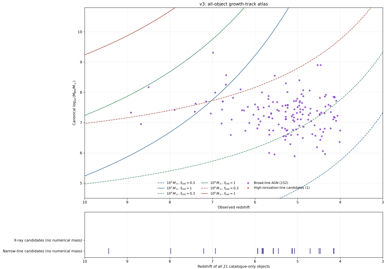
Figure 2. All 153 supported masses appear against reference tracks; the lower panel retains the redshifts and classes of all 21 no-inference objects.
