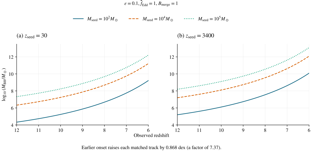
Figure 7: Growth from z_{\text{seed}} = 30 (a) and 3400 (b), with matched seed masses and the fixed assumptions shown. Earlier onset adds 99.90 Myr and shifts each track upward by 0.868 dex. Here z_{\text{seed}} denotes the assumed start of accretion. The z = 3400 comparison extrapolates the matter-plus-Lambda cosmology and assumes uninterrupted accretion. Radiation, gas supply, halo assembly and feedback are omitted.
