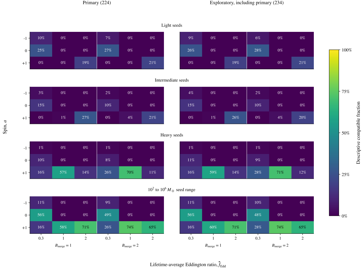
Figure 4: Constant-state compatibility fractions in the primary sample (left) and the inclusive exploratory sample (right). The exploratory sample includes all primary objects. Each column specifies merger multiplier B and fixed luminosity ratio f ; rows specify ideal spin-dependent efficiency, with the supercritical prescription in Appendix C. Seed intervals overlap and have no assigned probability weights. The broad mass interval spans several possible seed-formation channels.
