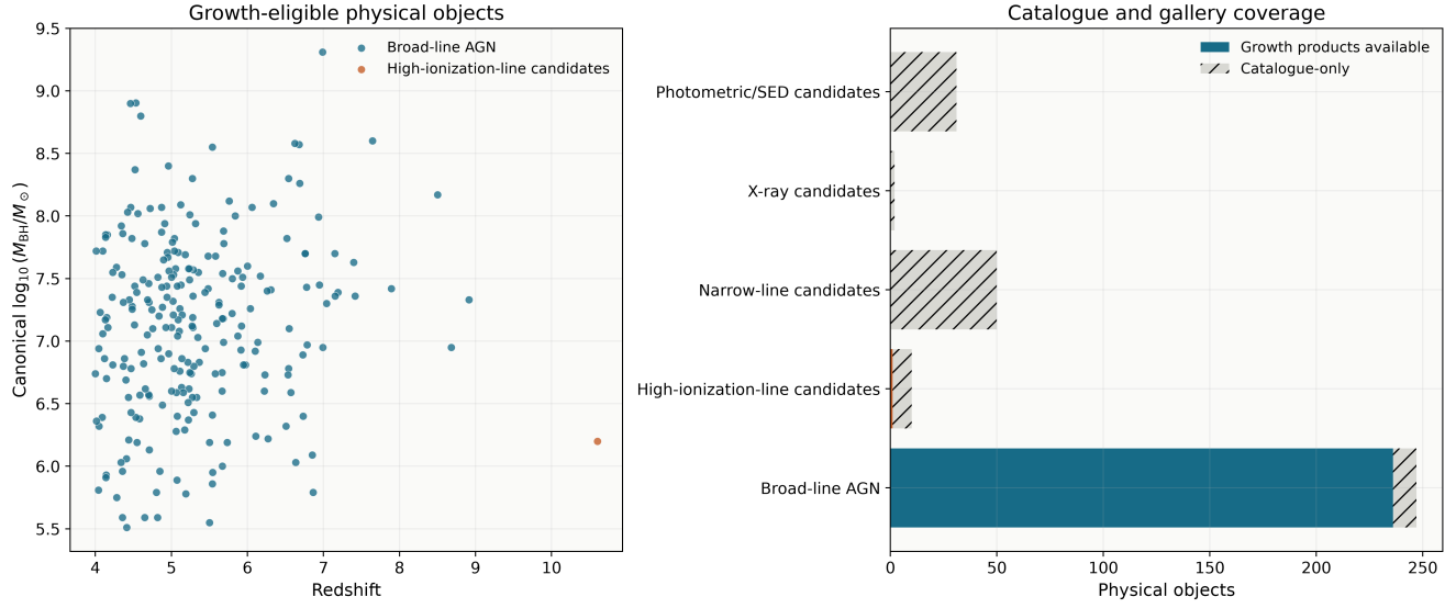
Figure 1: Catalogue landscape. Left: the 237 growth-eligible physical objects in black-hole-mass-redshift space. Right: product coverage for all 340 objects. The 103 catalogue-only objects remain available for provenance and evidence analysis without unsupported numerical growth products.
