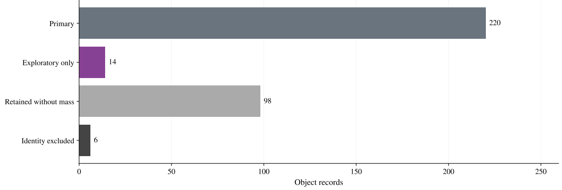
Figure 5: Sample accounting for 338 catalogue object records. Mutually exclusive categories comprise 220 primary objects, fourteen additional exploratory objects, 98 retained without eligible masses, and six identity exclusions. The inclusive exploratory numerical sample contains 234 objects.
