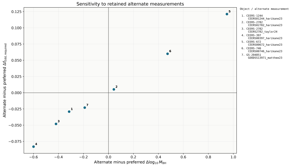
Figure 5: Seven alternate-measurement comparisons across six objects. Numbered points are keyed to stable object and measurement identifiers.
