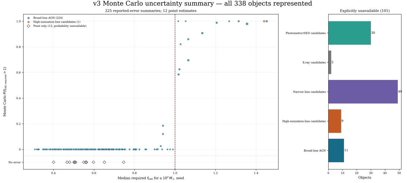
Figure 3: Exploratory-sample uncertainty summary for 225 objects with reported mass errors and 12 point estimates without mass errors, shown as open diamonds on the “No error” row. Point size encodes the 16th–84th percentile width for sampled objects. The accounting panel retains all 101 catalogue-only objects.
