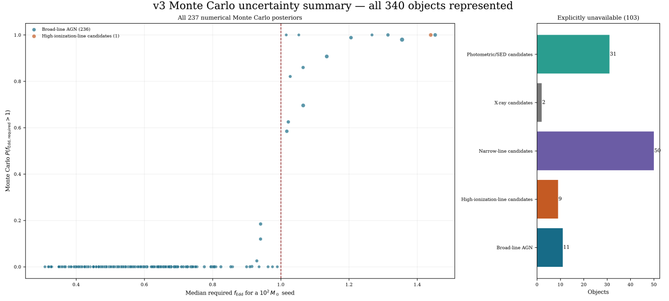
Figure 5: Complete Monte Carlo uncertainty summary. Every one of the 237 numerical posteriors is plotted; point size encodes the 16th–84th percentile width. The adjacent accounting panel retains all 103 catalogue-only objects. The full supplement atlas gives every object label and interval.
