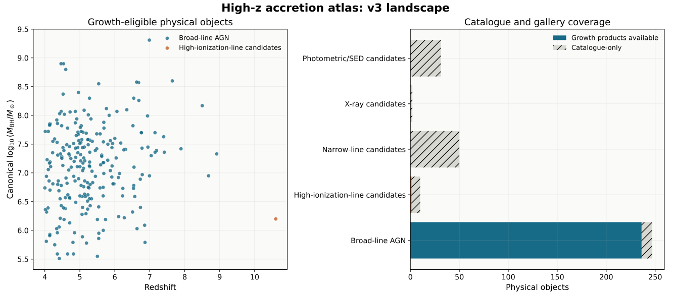
Figure 1: Current catalogue landscape. Left: all 237 growth-eligible physical objects in black-hole-mass–redshift space. Right: growth-product coverage for all 340 objects. The 103 catalogue-only objects remain available for provenance and evidence analyses but are not assigned numeric growth products.
