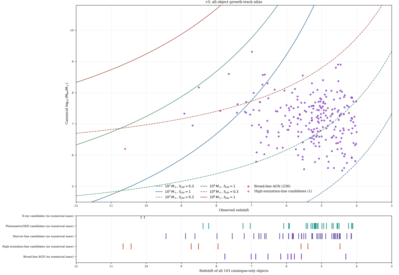
Figure 2: Complete v3 growth-track view. All 237 objects with supported canonical black-hole masses are plotted against reference tracks. The lower panel retains the redshift locations of all 103 catalogue-only objects for which a numerical growth history cannot be inferred. Thus every physical object is visible without assigning unsupported masses. The common reversed redshift axis spans z = 12 to z = 3 , centering the observed sample while retaining the original figure dimensions and margins. Broad-line AGN are purple.
