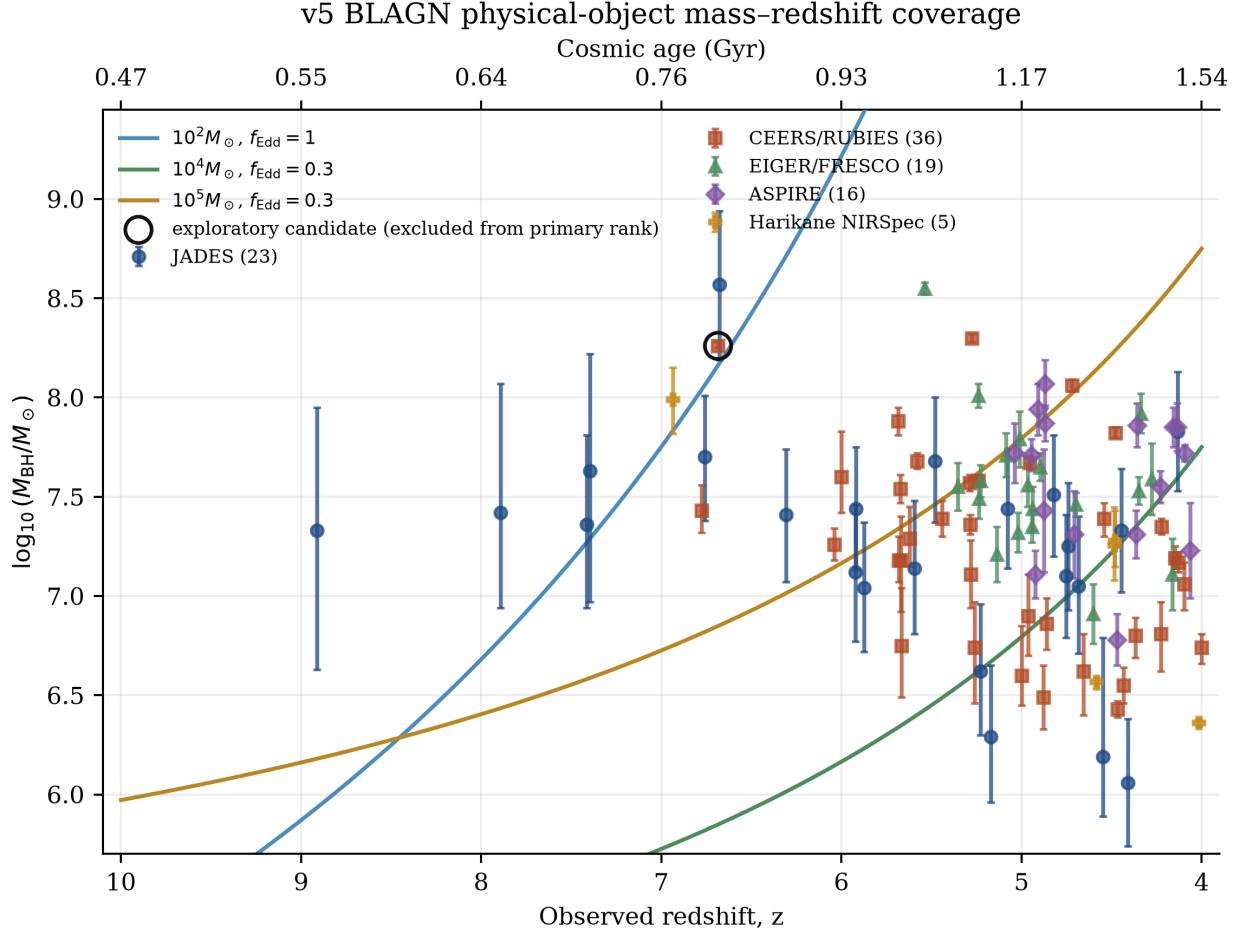
Figure 3: Current v5 physical-object mass-redshift coverage, stratified across the five preferred-measurement source selections. The open marker identifies the retained alternative-interpretation candidate excluded from the primary rank. Reference tracks use the repository baseline and are diagnostic rather than fitted histories.
