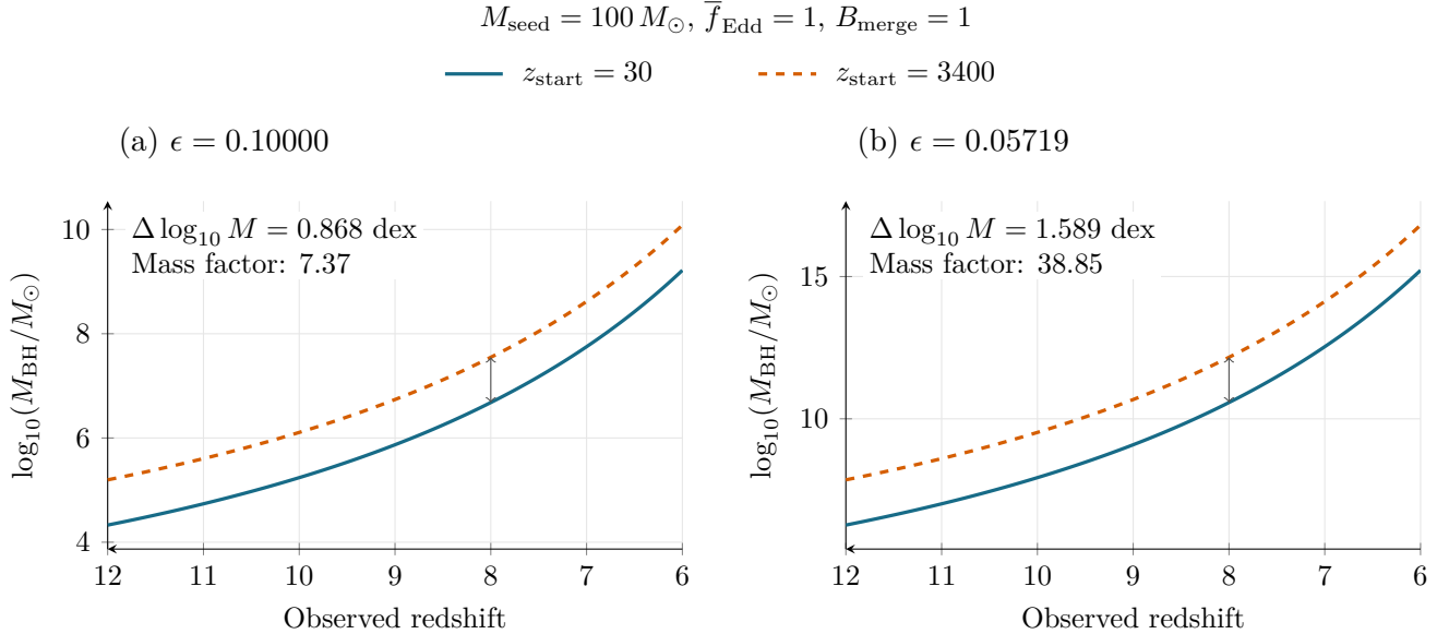
Figure 7: Effect of moving the start of otherwise identical accretion histories from z = 30 (solid blue) to 3400 (dashed orange). Both panels use M_{\text{seed}} = 100 M_\odot , \overline{f_{\text{Edd}}} = 1 and no merger boost; the fixed radiative efficiencies are 0.1 (a) and 0.05719 (b). Arrows mark the constant logarithmic mass offset from the additional 99.90 Myr of growth. The panels have different vertical ranges and show 6 \leq z \leq 12 to focus on early growth. These are controlled analytic comparisons, not fitted histories. The z = 3400 curves extrapolate the matter-plus-Lambda age relation and assume uninterrupted accretion; they do not model PBH formation or establish that such early gas accretion occurs.
