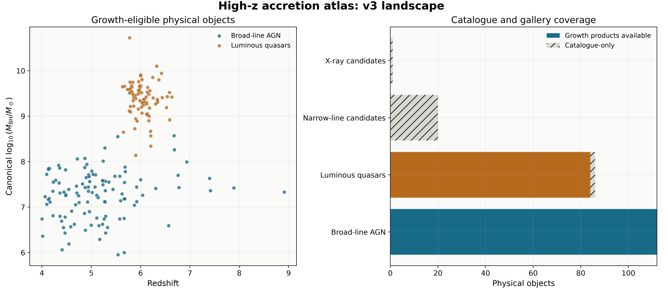
Figure 1: Current catalogue landscape. Left: all 196 growth-eligible physical objects in black-hole-mass–redshift space. Right: growth-product coverage for all 219 objects. The 23 catalogue-only objects remain available for provenance and evidence analyses but are not assigned numeric growth products.
