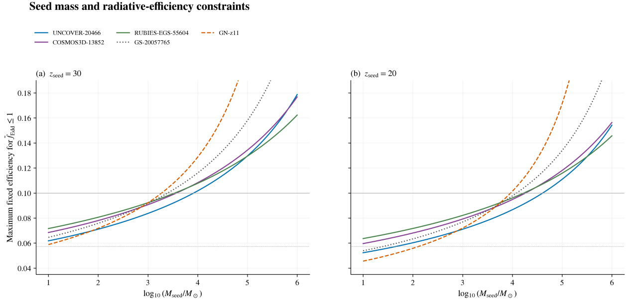
Figure 3: Seed-mass–efficiency boundaries for Eddington-limited average growth at two starting redshifts. Each curve uses an adopted point mass and no merger boost. Below a curve the required average is at most unity. Horizontal guides mark \epsilon = 0.1 (solid grey) and 1 - \sqrt{8/9} (dotted grey). GN-z11 (dashed) is exploratory; the other objects are primary. These are fixed-efficiency comparisons without probability weights.
