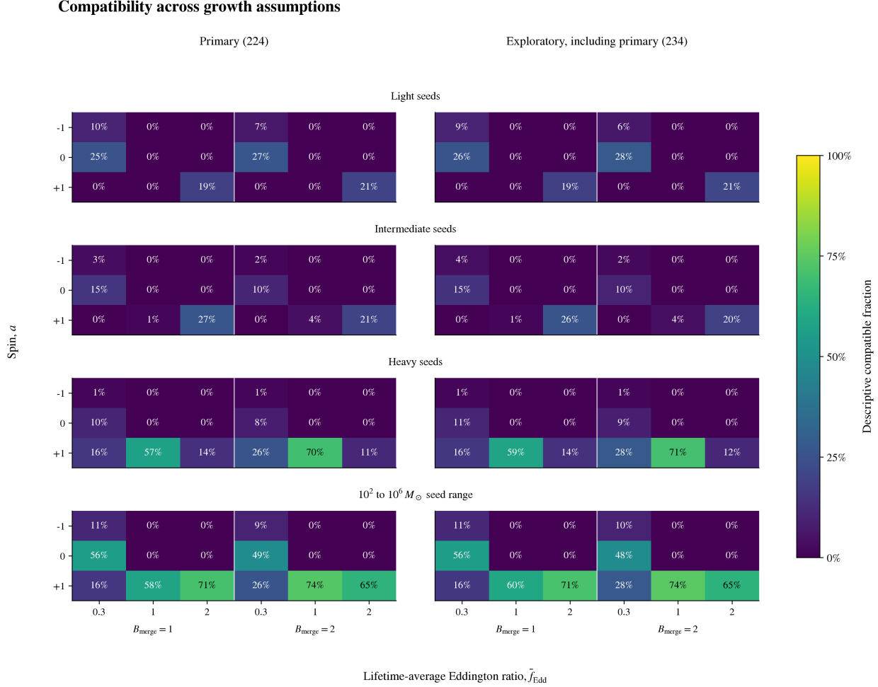
Figure 4: Constant-state compatibility fractions in the primary sample (left) and the inclusive exploratory sample (right). These samples are nested. Each column specifies merger multiplier B and fixed luminosity ratio f ; rows specify ideal spin-dependent efficiency, with the supercritical prescription in Appendix C. Seed intervals overlap and carry no probability weights. The broad mass interval has no formation-channel interpretation.
