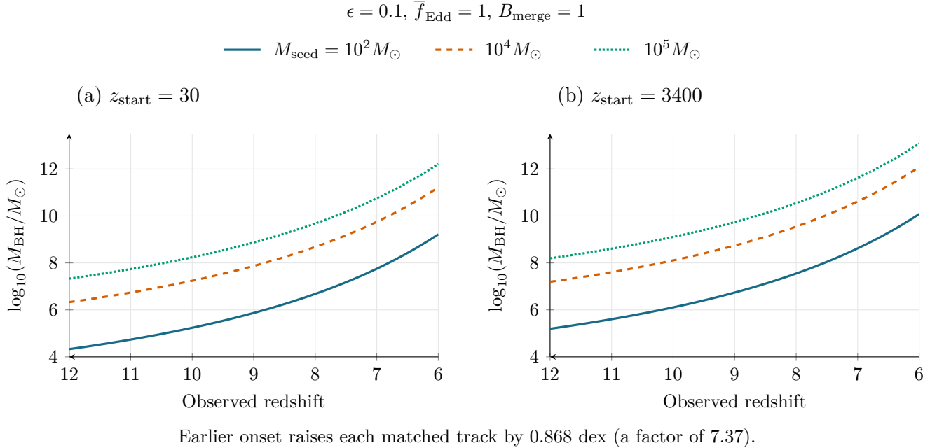
Figure 7: Matched growth tracks starting at z = 30 (a) and z = 3400 (b). Colours and line styles identify seeds of 10^2 , 10^4 and 10^5 M_\odot ; all tracks use \epsilon = 0.1 , \overline{f_{\text{Edd}}} = 1 and no merger boost. Both panels use identical axis limits. Moving the start earlier adds 99.90 Myr and raises every matched track by 0.868 dex (a factor of 7.37), without changing its shape. The displayed range 6 \leq z \leq 12 focuses on early growth. These are controlled analytic comparisons, not fitted histories. The z = 3400 curves extrapolate the matter-plus-Lambda age relation and assume uninterrupted accretion; they do not model PBH formation or establish that such early gas accretion occurs.
