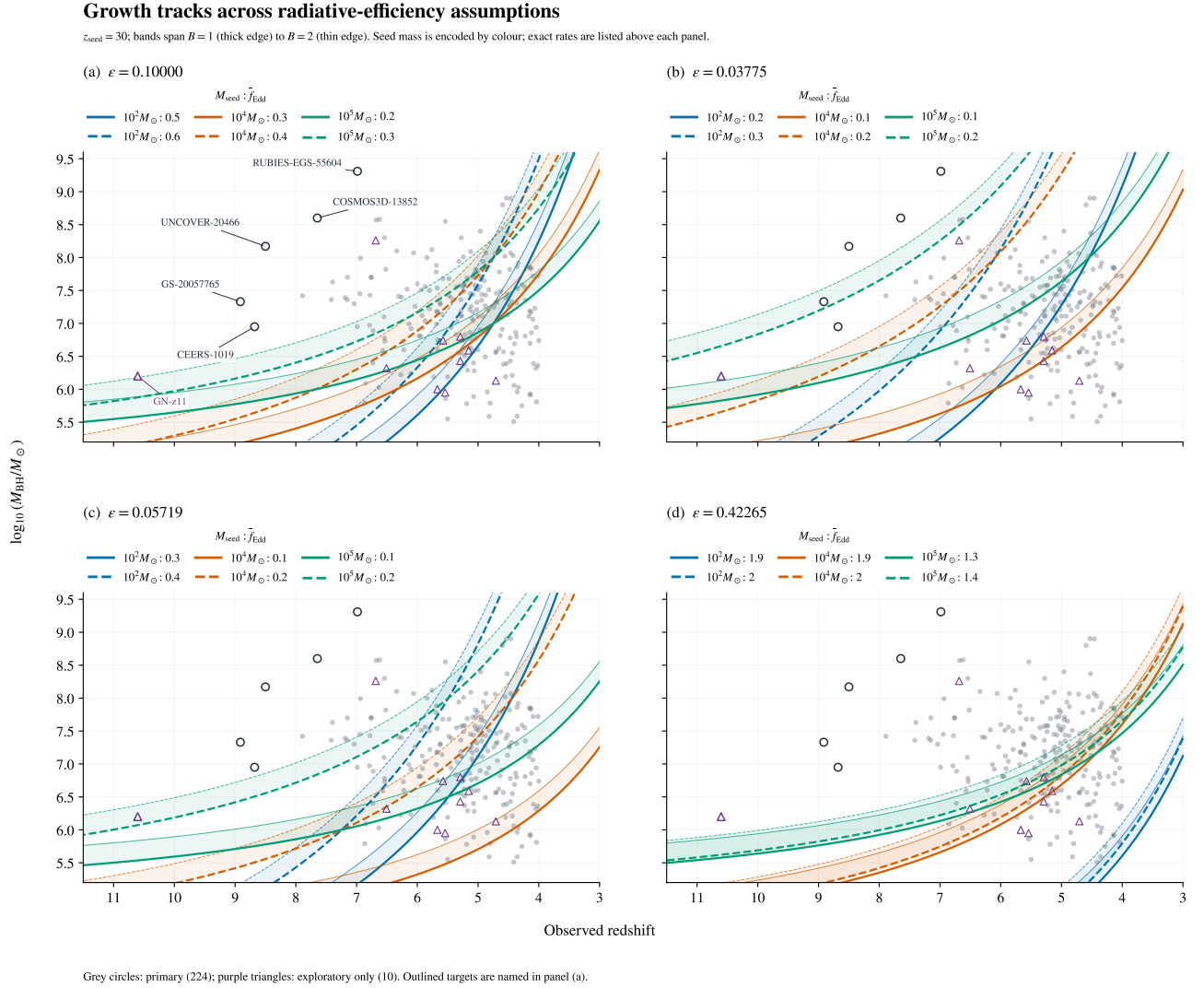
Figure 1: Growth tracks with 224 primary and ten exploratory-only objects. Panels show four constant radiative efficiencies at z_{\text{seed}} = 30 ; colours distinguish seeds of 10^2 , 10^4 and 10^5 M_{\odot} , and legends list the selected average Eddington ratios. Shaded bands span merger boosts B = 1 – 2 , with thick and thin edges respectively. The bands show the effect of the assumed merger boost. Six named objects are outlined in every panel. The reversed redshift axis spans z = 11.5 to z = 3 . Excluded identities and objects without eligible masses are omitted.
