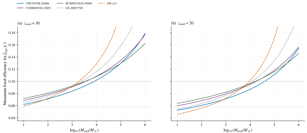
Seed mass and radiative-efficiency constraints
