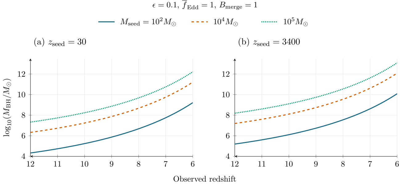
Figure 7: Growth from z_{\text{seed}} = 30 (a) and 3400 (b), with matched seed masses and the fixed assumptions shown. Earlier onset adds 99.90 Myr and shifts each track upward by 0.868 dex. Here z_{\text{seed}} marks the start of accretion, not necessarily PBH formation. The z = 3400 comparison extrapolates the matter-plus-Lambda cosmology and assumes uninterrupted accretion; it is not a physical model of PBH evolution.
