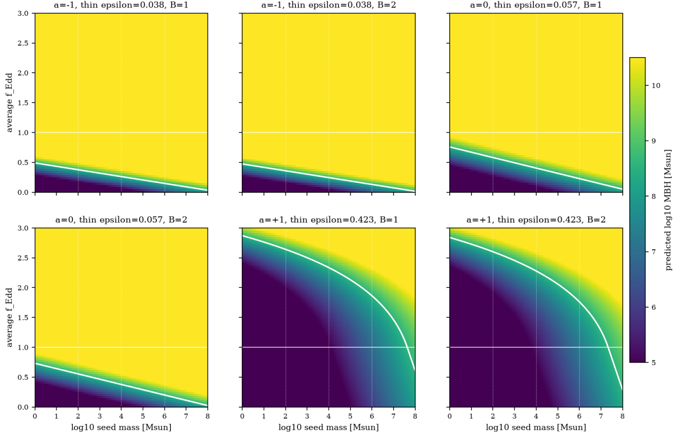
Figure 6. GN-38509 f_{\text{Edd}} -mass sheet. Six spin/merger combinations show which seed and accretion choices reproduce the preferred mass.
