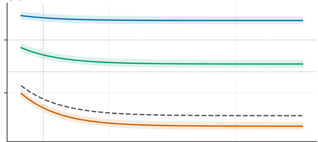
(b) COSMOS3D-13852
