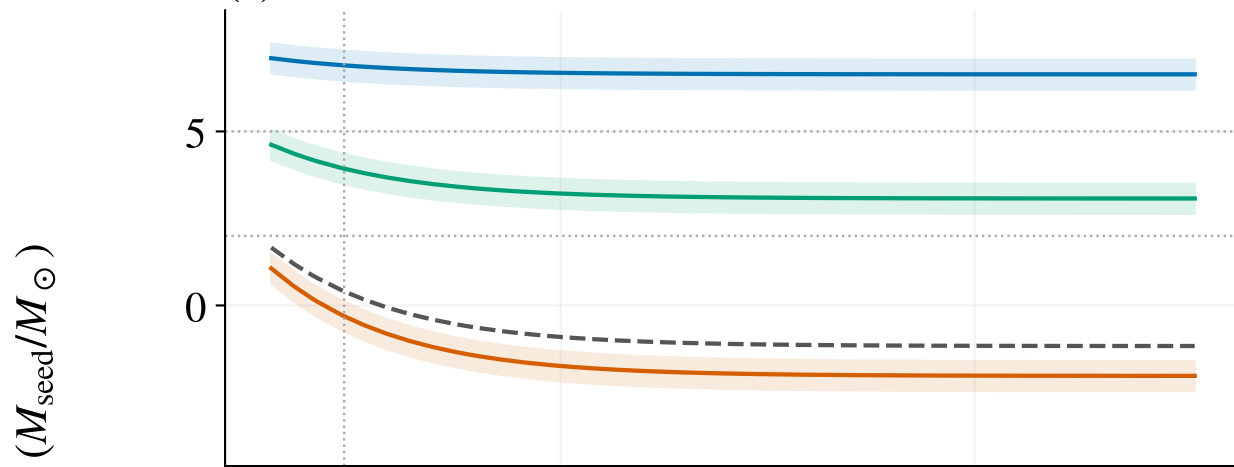
(a) UNCOVER-20466
