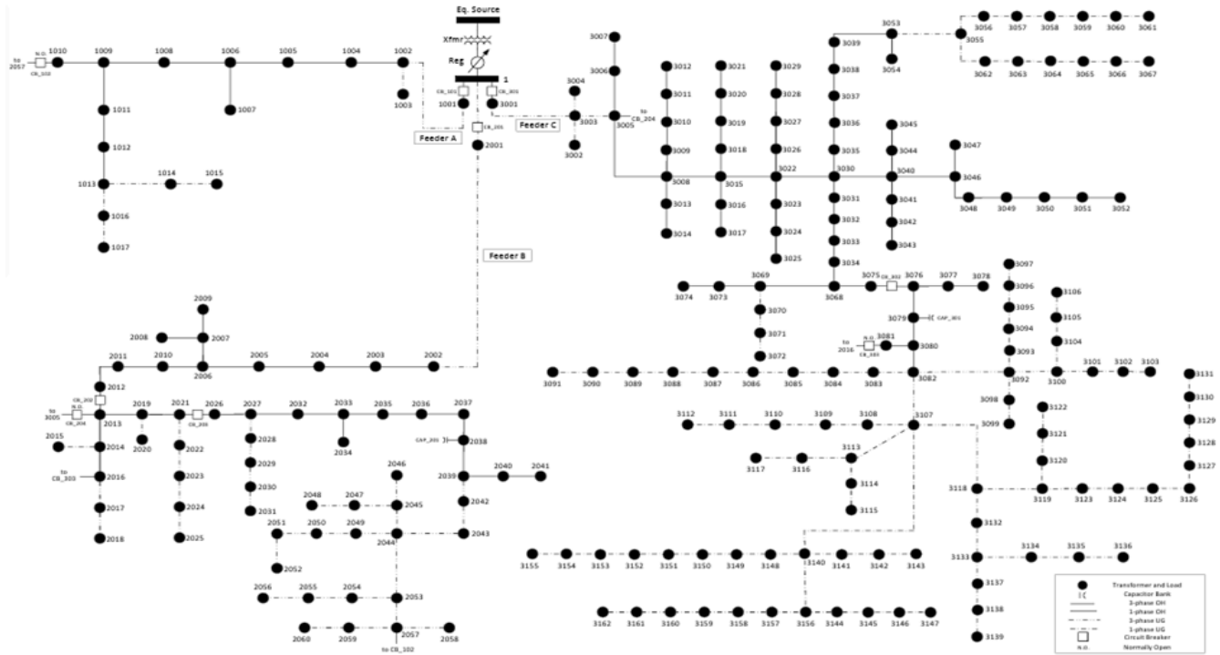
Figure 1 - Bus Distribution Test System for the dataset
