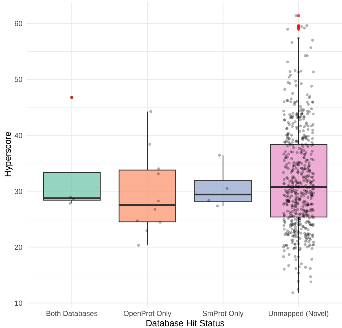
MS/MS Identification Quality across Databases
