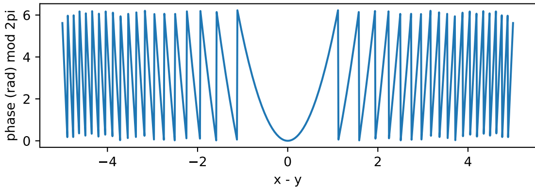
Free-particle propagator phase ( m=1, \hbar=1, dt=0.1 )
