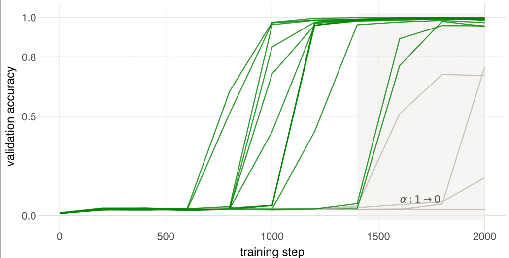
Anneal to raw read (shaded): 12/16 finish as stock mLSTMs
