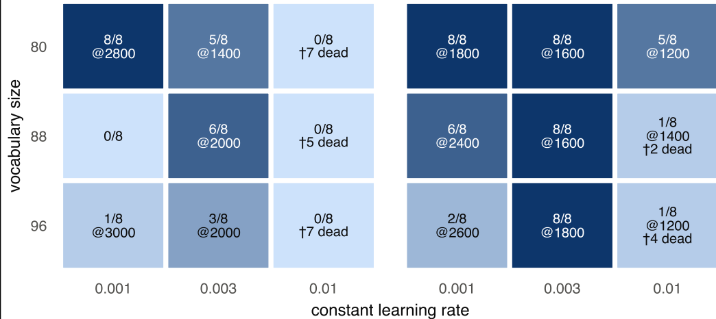
Basin map: solved/8 (3000 steps, seq 768); † = destabilized
