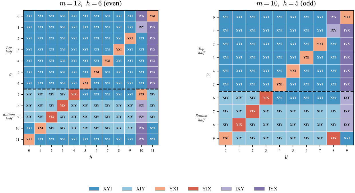
Figure 4: Staircase layer (penultimate, s = m-2 ) for m = 12 ( h = 6 , even) and m = 10 ( h = 5 , odd). Each cell is colored by its direction triple. The top half shows the diagonal walk ( YXI descending one column per row, IYX anchoring the last column). The bottom half exhibits different patterns depending on the parity of h . The dashed line separates the two halves at row h .
