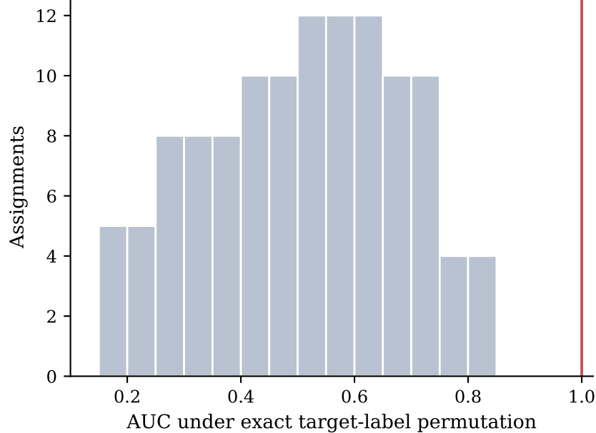
a Exact permutation null
