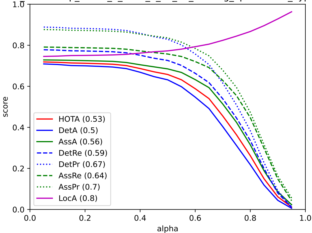
2x_data_source-clip_based_2_class_2_11_25_training_epochs-500_hyperpara
