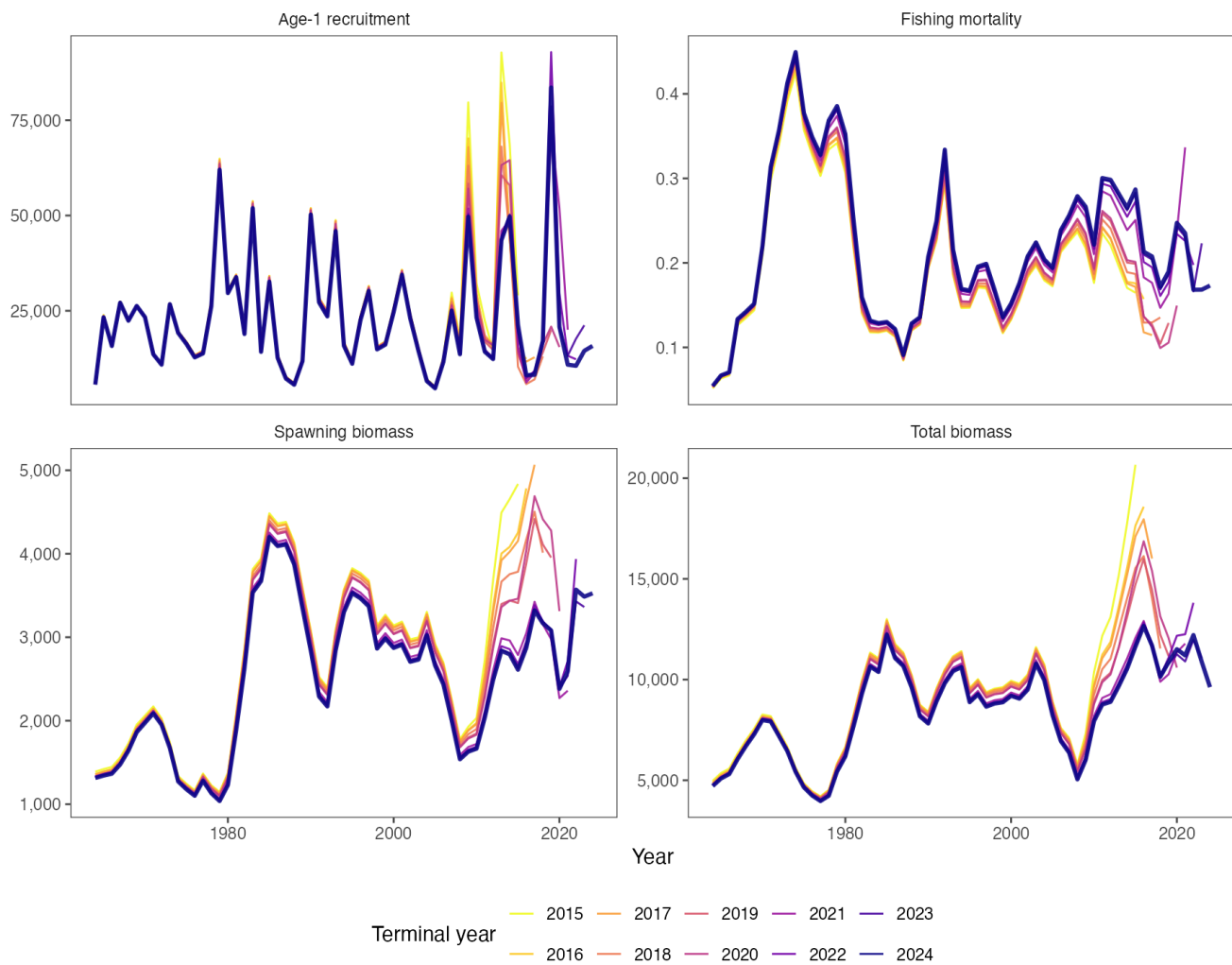
Figure 20: Spawning biomass, total biomass, recruitment, and fishing mortality for Model 26.0 and nine lag-preserving retrospective peels.
