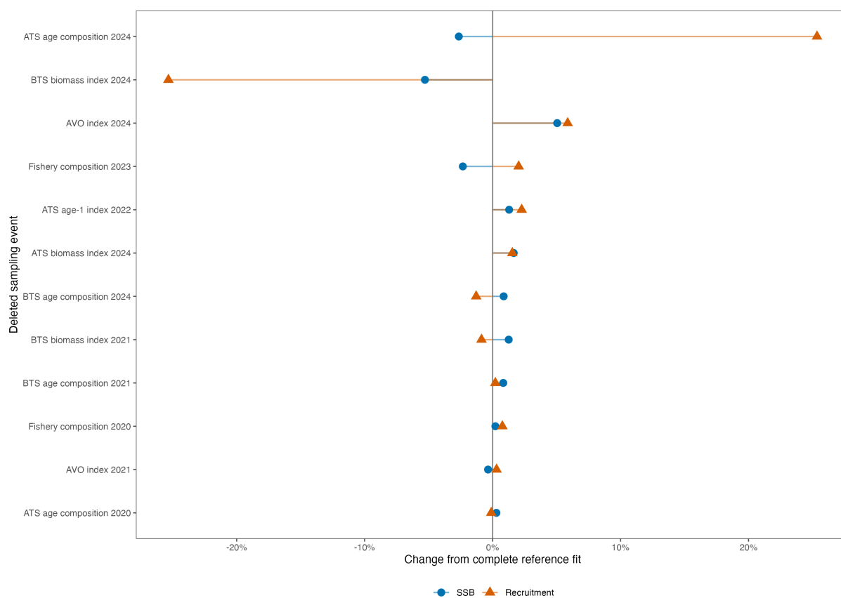
Figure 30: Influence of selected sampling-event deletions on terminal spawning biomass and age-1 recruitment.
