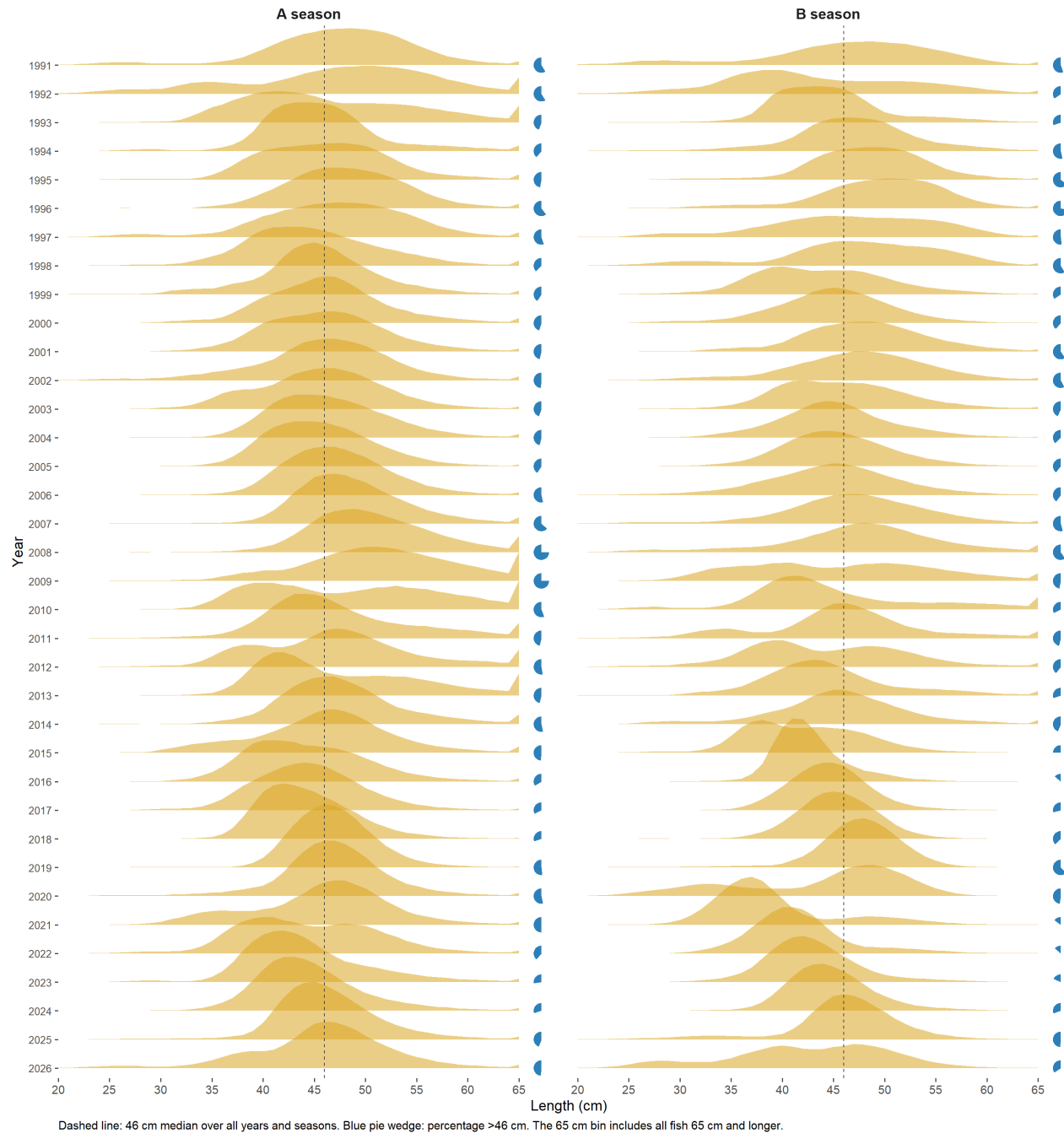
Figure 31: Pollock length-frequency proportions by season. The left panel shows samples collected before June 20; the right panel shows samples collected from June 20 onward.
