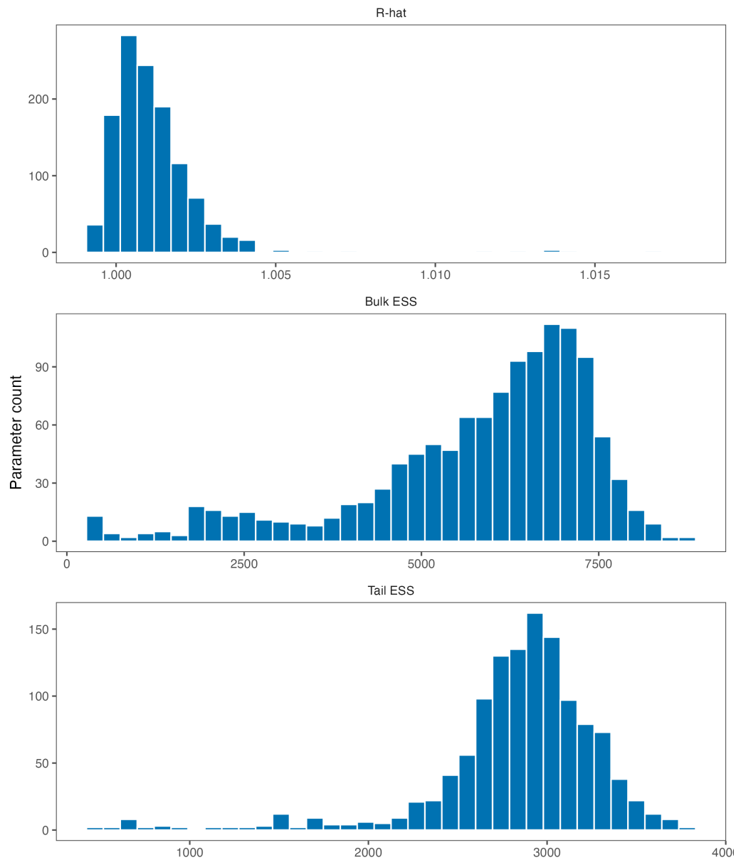
Figure 28: Distributions of R-hat, bulk ESS, and tail ESS across the 1,218 sampled parameters.
