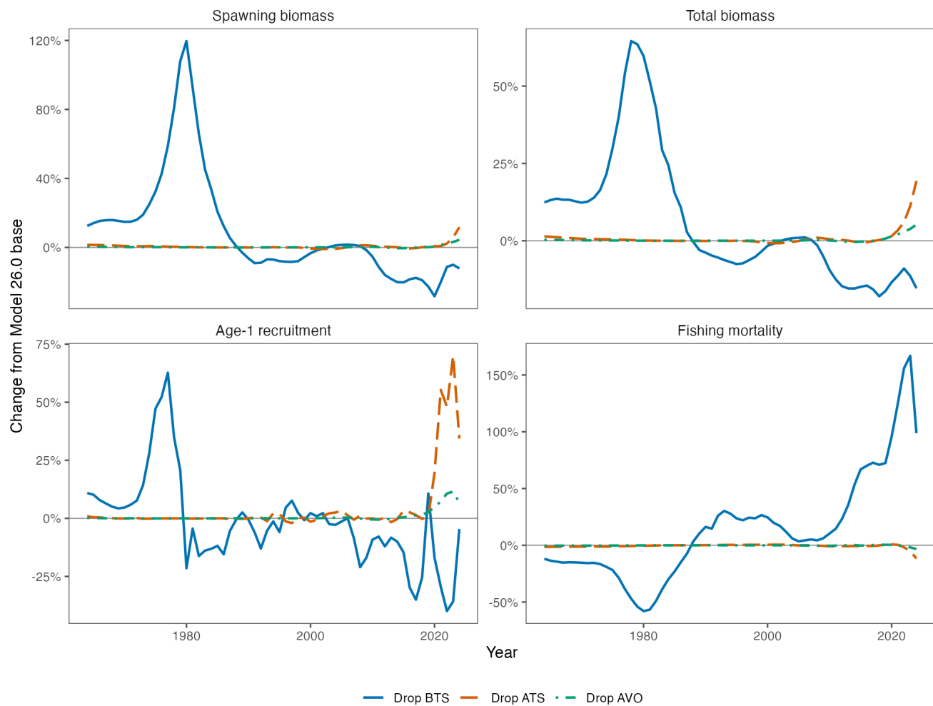
Figure 19: Annual changes in spawning biomass, total biomass, age-1 recruitment, and fishing mortality after dropping the complete BTS, ATS, or AVO fleet from Model 26.0.
