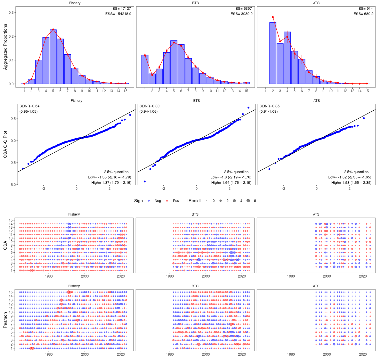
Figure 16: Aggregate age-composition fits, OSA quantile plots, and residual bubbles for the fishery, BTS, and ATS. The fishery and BTS panels retain every input year. ATS uses ages 2–15 and retains 18 display years because its sample size of one in 2020 produces zero rounded counts in the plotting conversion.
