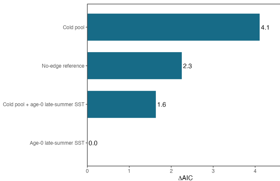
Figure 25: AIC differences among the four current-branch DSEM recruitment models.
