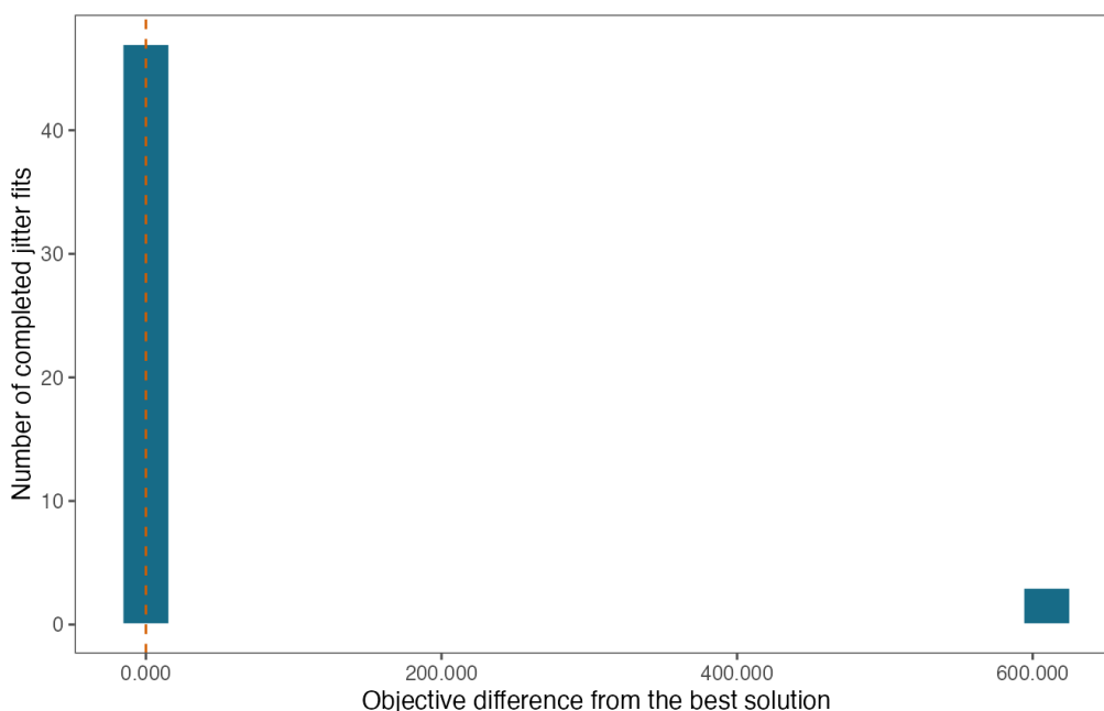
Figure 17: Distribution of objective differences from the best solution in 50 jitter refits.
