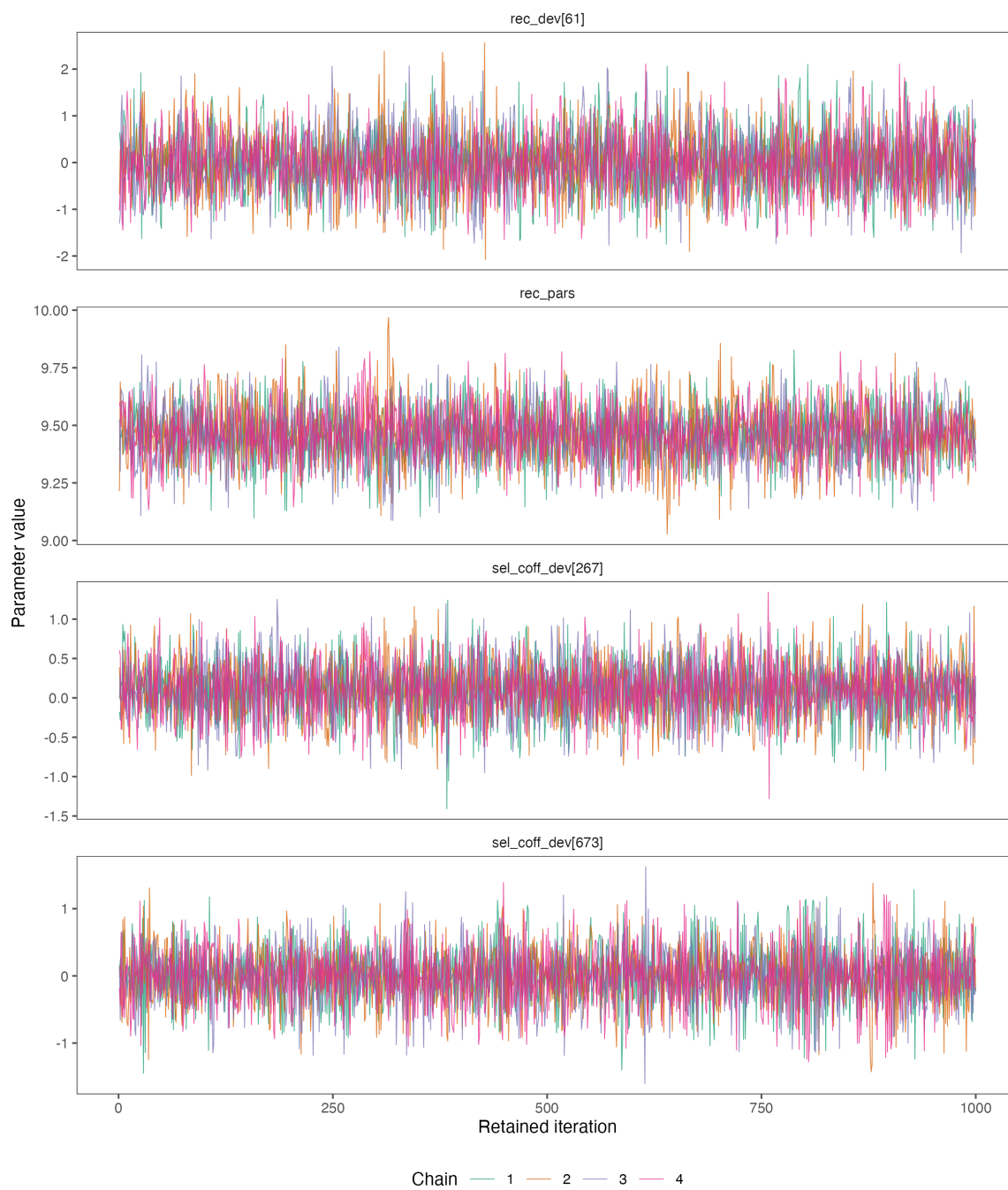
Figure 27: Retained SparseNUTS draws for four representative Model 26.0 parameters.
