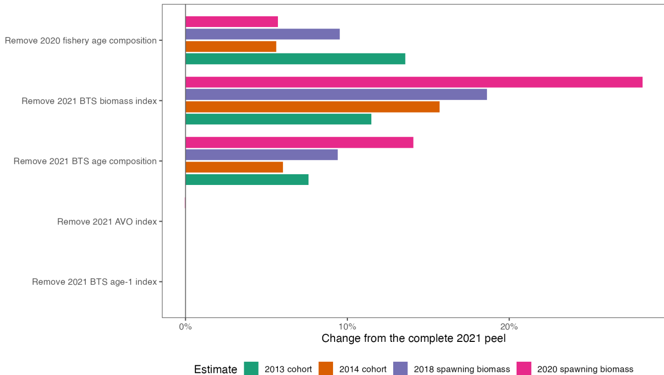
Figure 21: Influence of data blocks entering between the lag-preserving 2020 and 2021 peels.
