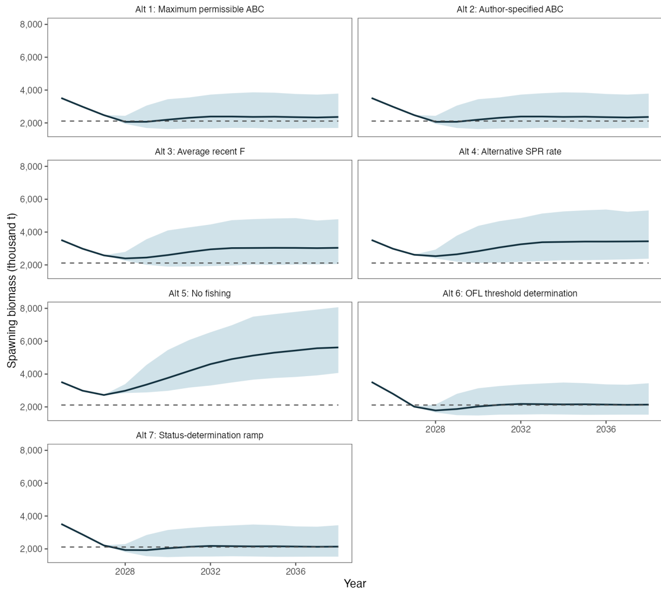
Figure 22: Projected spawning biomass under the seven Standard Projection Model alternatives.
