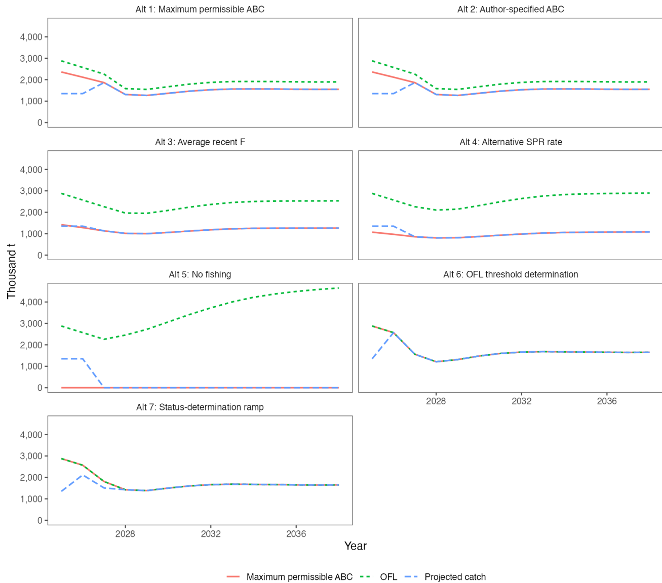
Figure 23: Projected catch, ABC, and OFL under the seven Standard Projection Model alternatives.
