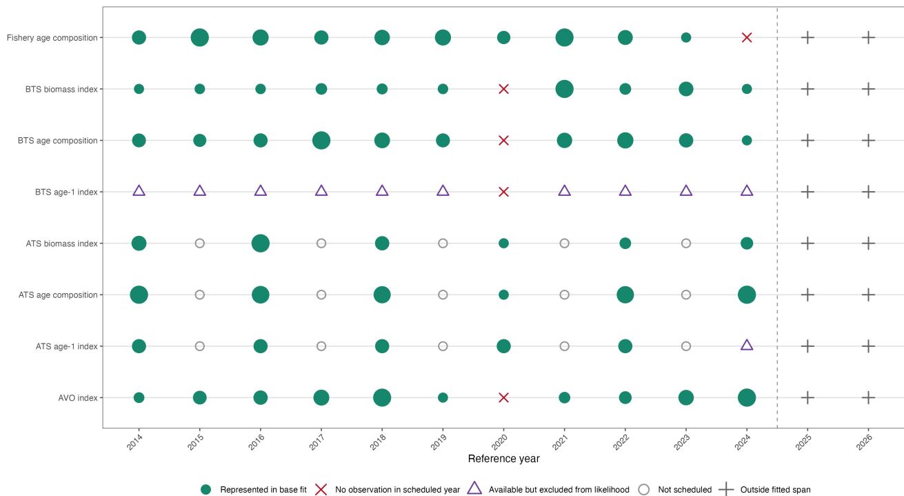
Figure 29: Observation continuity for fishery, BTS, ATS, and AVO inputs from 2014 through 2026.
