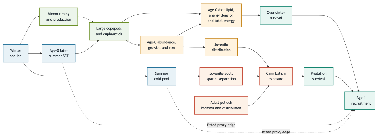
Figure 24: Conceptual pathways from physical conditions and prey through age-0 condition, overwinter survival, cannibalism, and age-1 recruitment.
