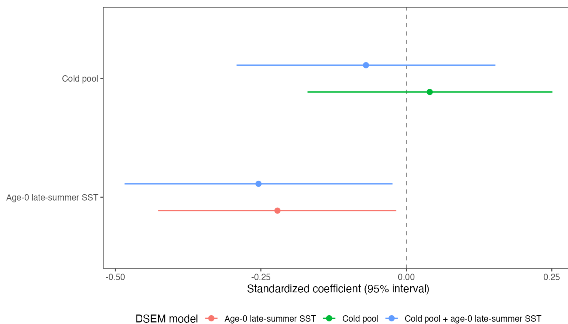
Figure 26: Standardized cold-pool and age-0 SST coefficients for the exploratory DSEM models.
