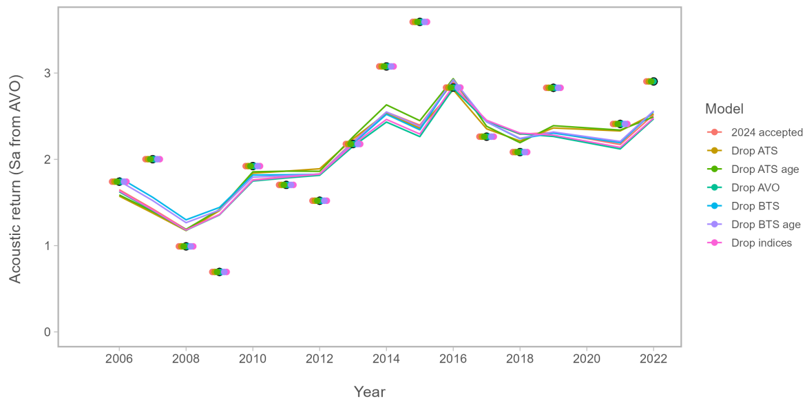
Figure 16: Comparison of fits to the Acoustic Vessels of Opportunity (AVO) biomass index for models that downweight one data source at a time
