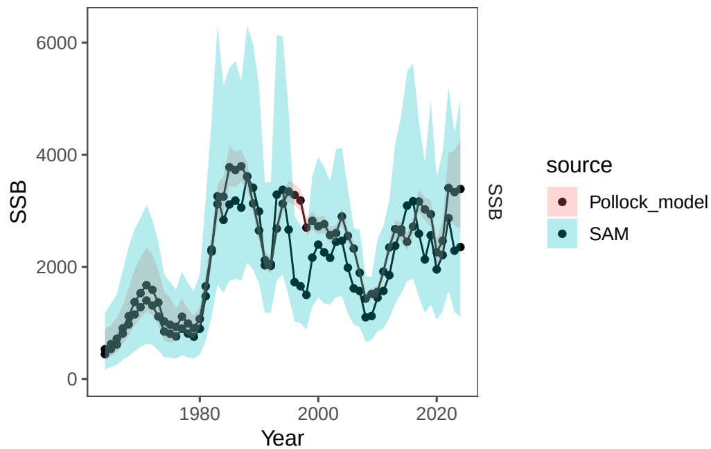
Figure 23: Model results comparing last year's model with the SAM model for spawning biomass (top) and recruitment at age 1 (bottom).
