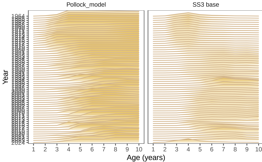
Figure 19: Model results comparing selectivity estimates between the base SS3 model configuration and the pollock model accepted in 2024.
