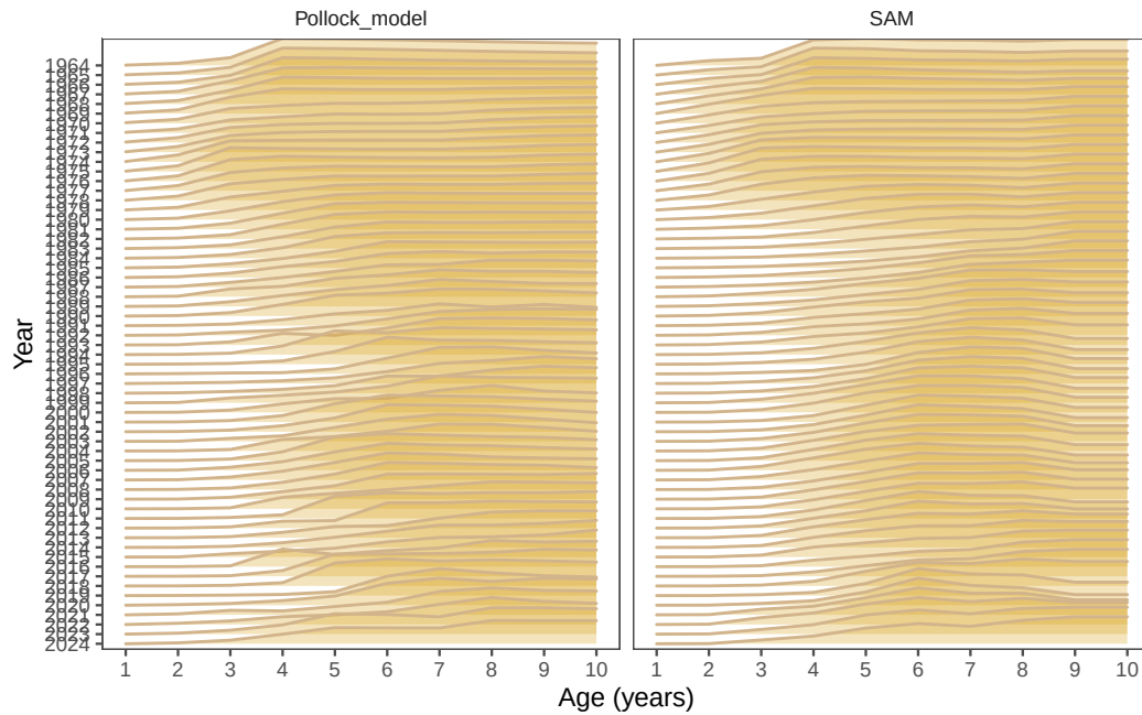
Figure 22: Model results comparing last year's model with the SAM model.
