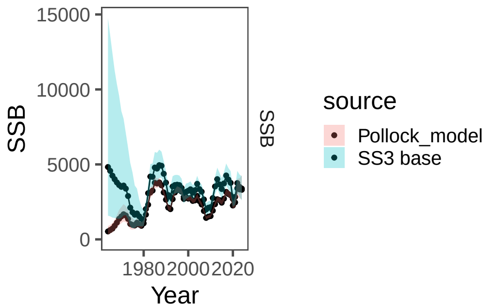
Figure 20: Model results comparing the base SS3 model configuration with the model used for pollock in 2024.
