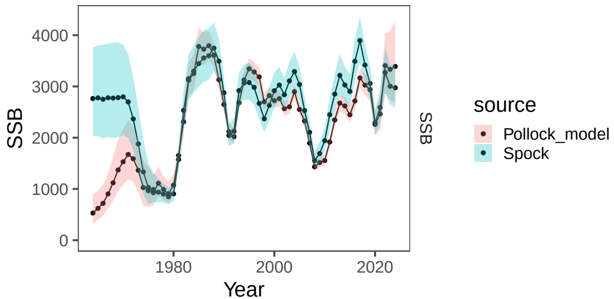
Figure 31: Model results comparing last year's model with the SPock model.
