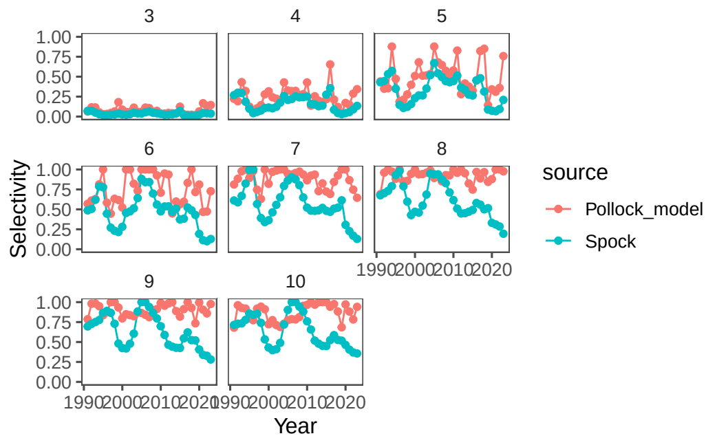
Figure 30: Model results comparing last year's model with the SPock model.
