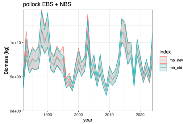
Figure 33: Model results comparing last year’s model with the revised sdmTMB model.
