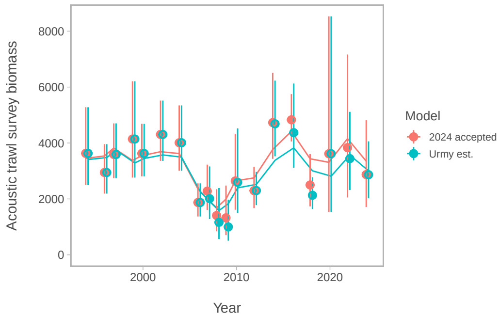
Figure 21: Comparison of fits to the Eastern Bering Sea acoustic-Trawl Survey (ATS) biomass index for the accepted 2024 model and one with revised estimates of index values and uncertainty from Urmy et al., (in prep).
