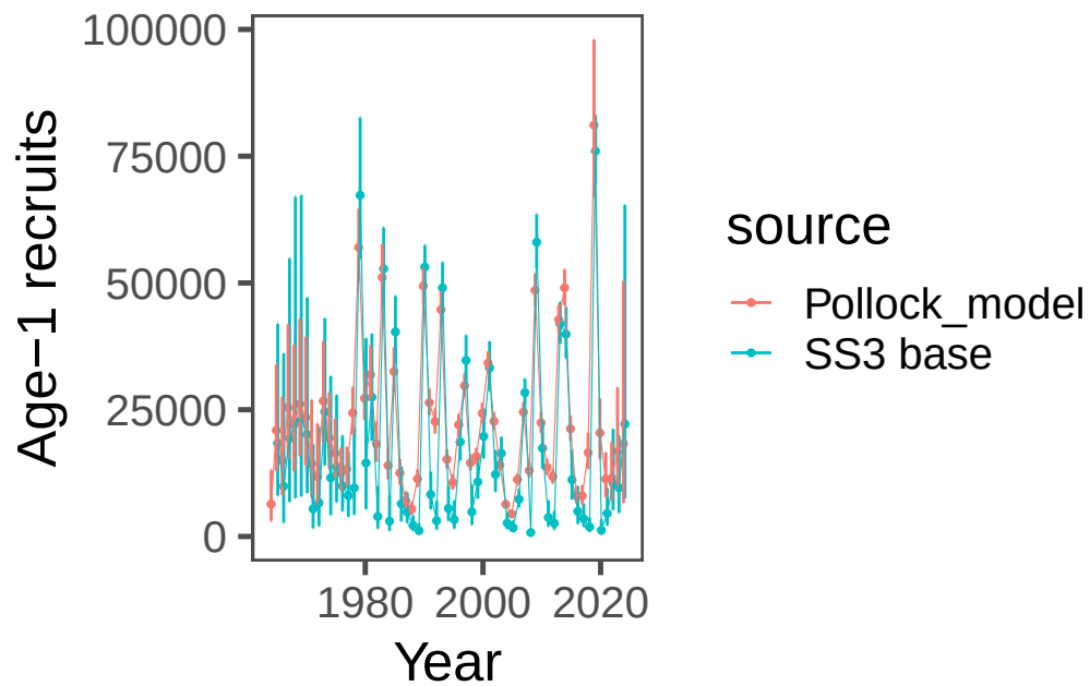
Figure 27: Model results comparing the base SS3 model configuration with the model used for pollock in 2024.
