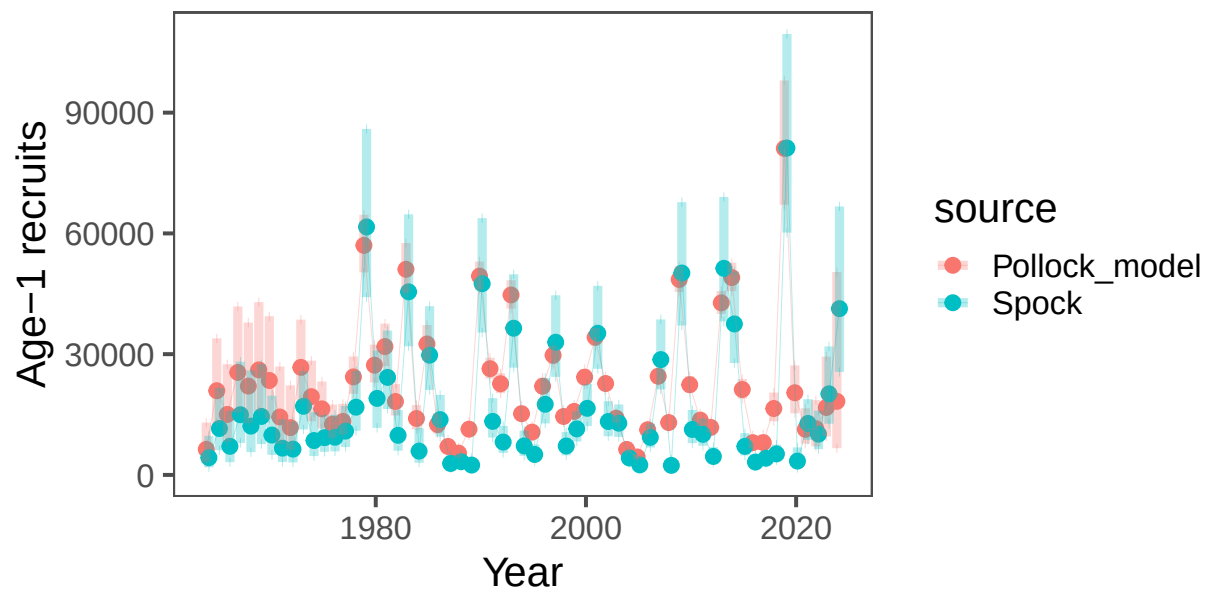
Figure 36: Model results comparing last year's model with the SPock model.
