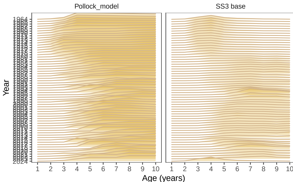
Figure 25: Model results comparing selectivity estimates between the base SS3 model configuration and the pollock model accepted in 2024.
