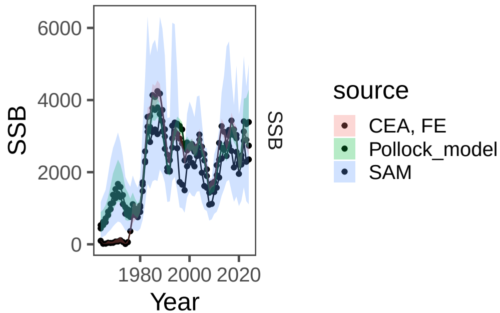
Figure 32: Model results comparing last year's model with the Rceattle model.
