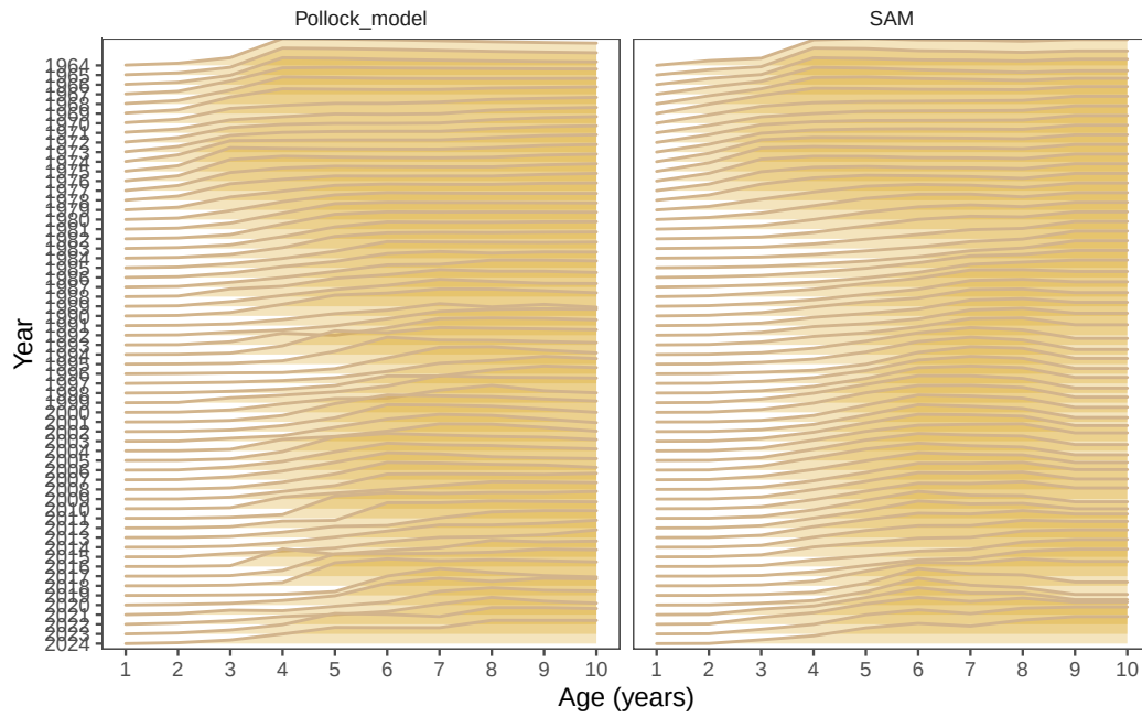
Figure 28: Model results comparing last year's model with the SAM model.
