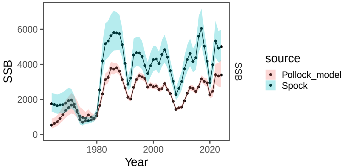
Figure 35: Model results comparing last year's model with the SPock model.
