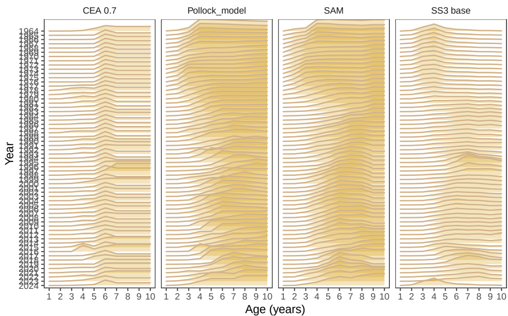
Figure 19: Model results comparing last year's model with the Rceattle model.
