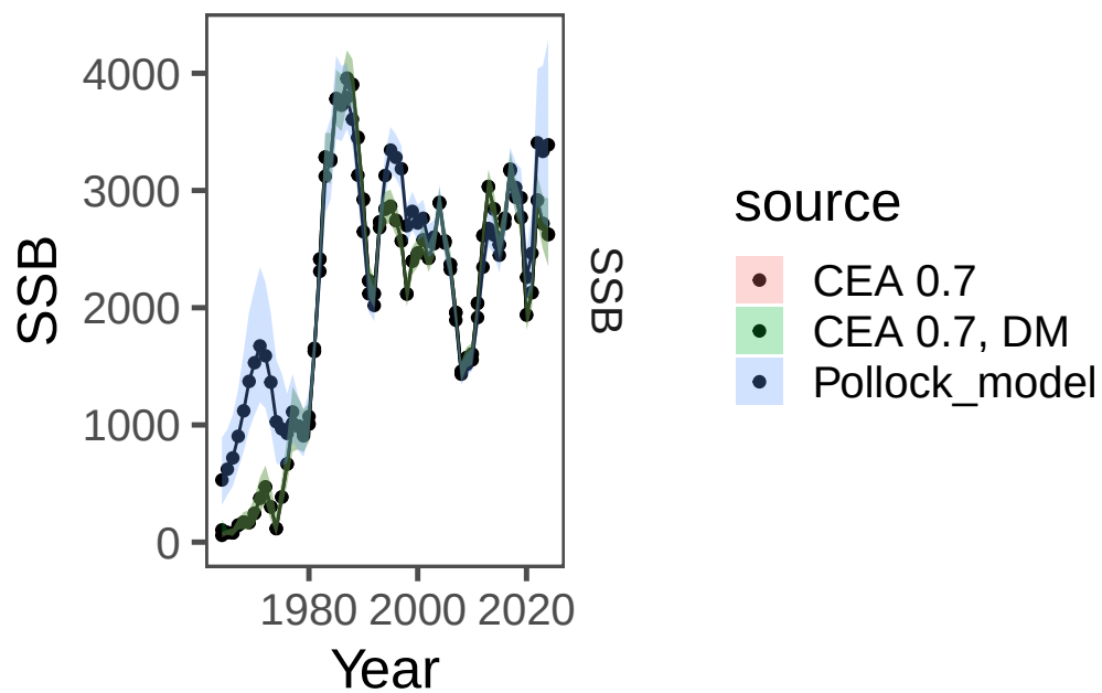
Figure 18: Model results comparing last year's model with the Rceattle model.
