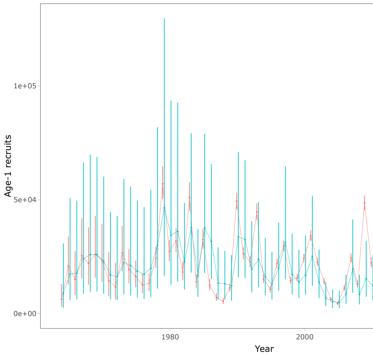
Figure 16: Model results comparing last year's model with the SAM model for spawning biomass (top) and recruitment at age 1 (bottom).
