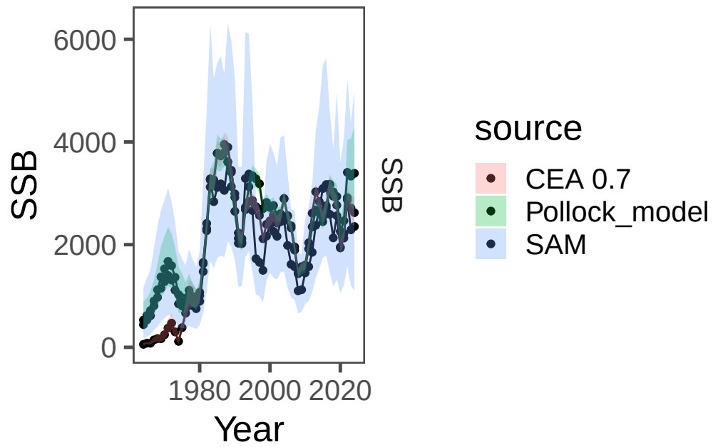
Figure 20: Model results comparing last year's model with the Rceattle model.
