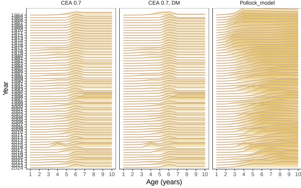
Figure 17: Model results comparing last year's model with the Rceattle model.
