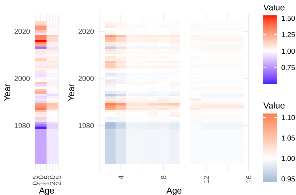
Figure 19: Depiction of the natural mortality (variability from mean value at age) as estimated from CEATTLE.
