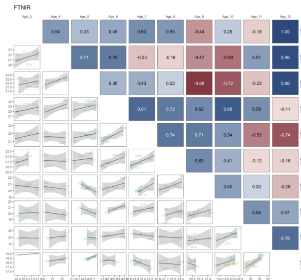
Figure 4: Cohort consistency over different ages based on log-abundance from the bottom-trawl survey data for pollock in recent years for FTNIRs age estimates. The cohorts are shown in the labels.
