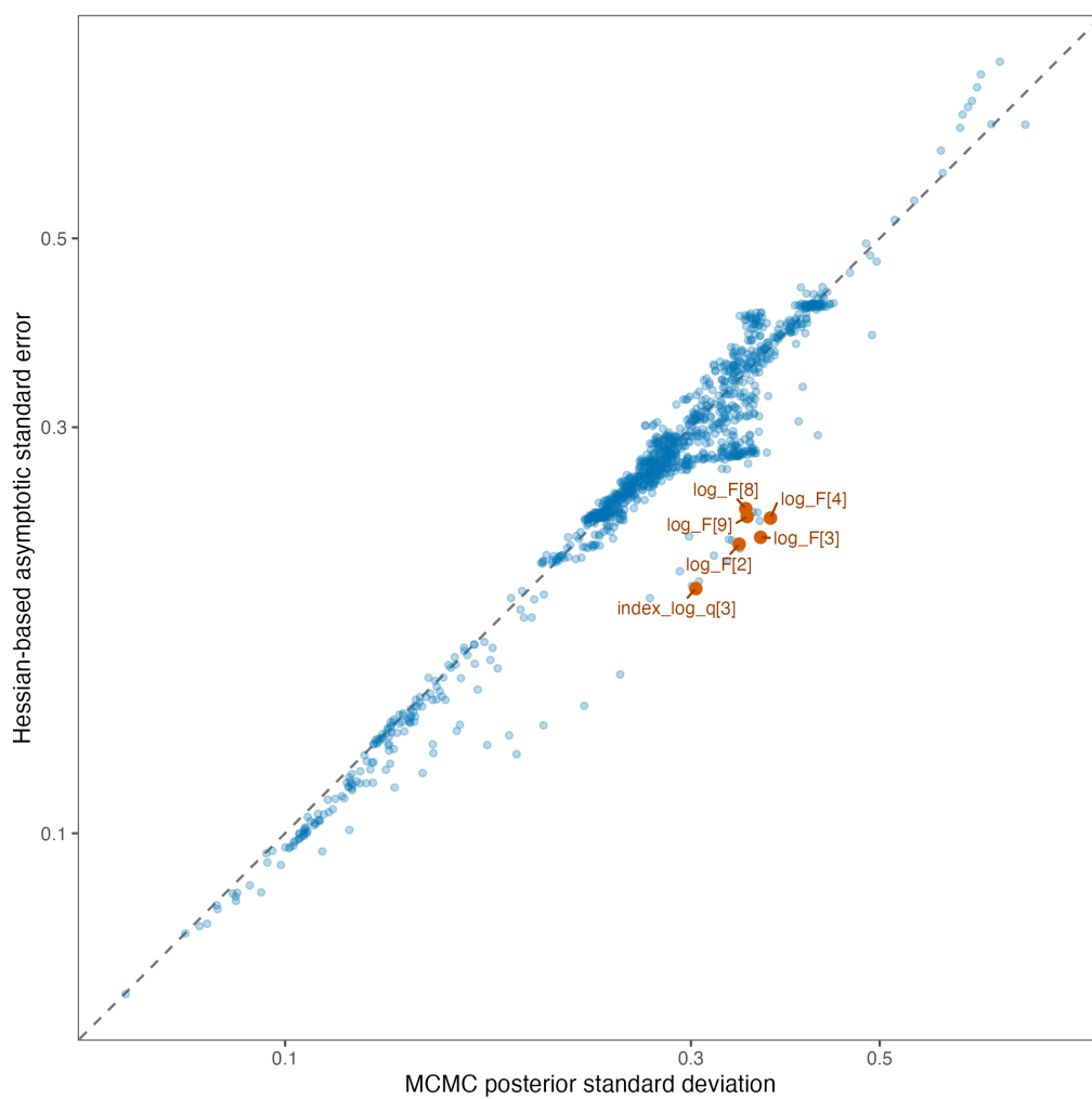
Figure 30: MCMC posterior standard deviations compared with Hessian-based asymptotic standard errors for all 1,218 Model 26.0 parameters.
