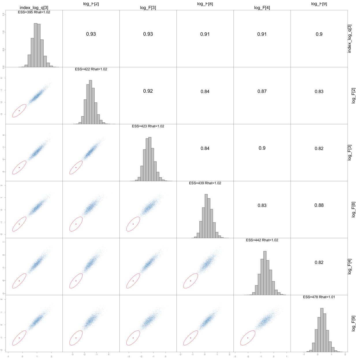
Figure 29: Joint posterior relationships for the six Model 26.0 parameters with the lowest bulk effective sample sizes. Diagonal panels report bulk ESS and R-hat; upper panels report posterior correlations; and lower panels show retained draws in blue, the maximum-likelihood estimate as a red point, and the local 95% Hessian ellipse in red.
