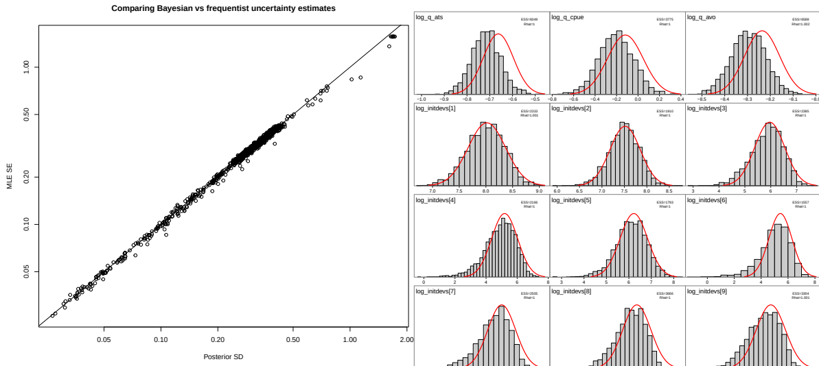
(a) Comparison of posterior marginal standard deviation with the asymptotic approximation.
