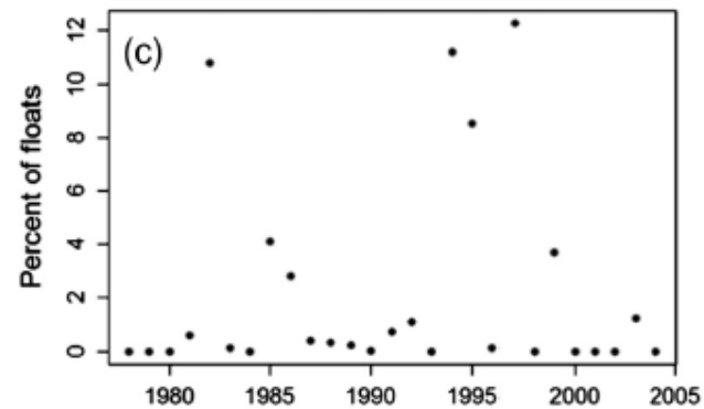
2°W advection
