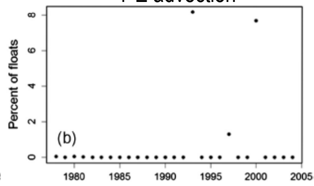
1°E advection
