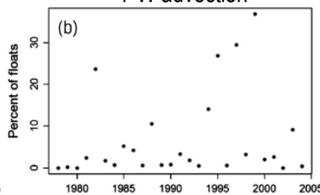
1°W advection
