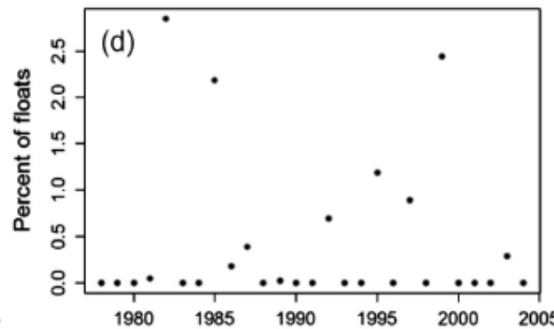
3°W advection
