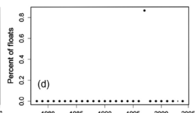
3°E advection
