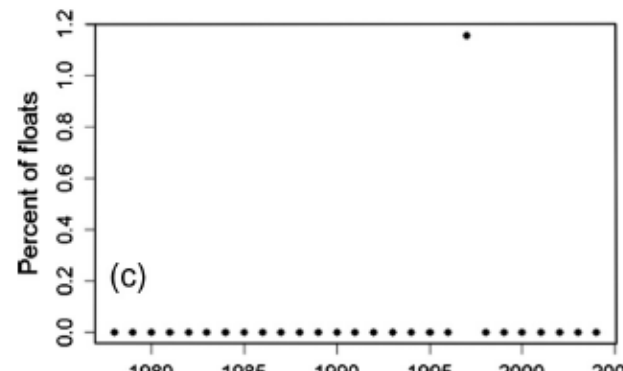
2°E advection
