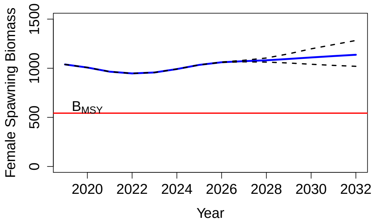
Figure 4.28: Projected female spawning biomass for 2019 to 2032 (blue line), with 5% and 95% confidence intervals, and fishing at the 5-year (2014-2018) average fishing mortality rate, F = 0.0714 , Model 18.2.
