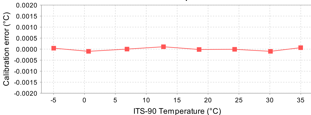
Calibration error vs. Temperature
