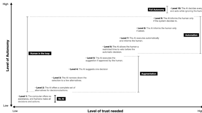
Fig. 19. levels of automation [41]
