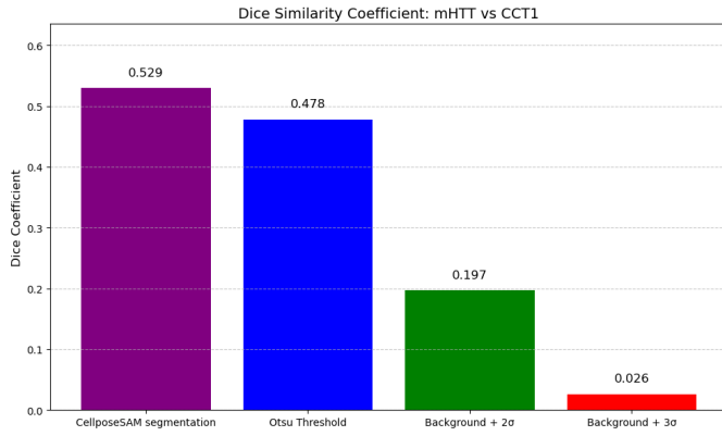
Fig. 10. Dice coefficient barplot for segmentation comparison.
