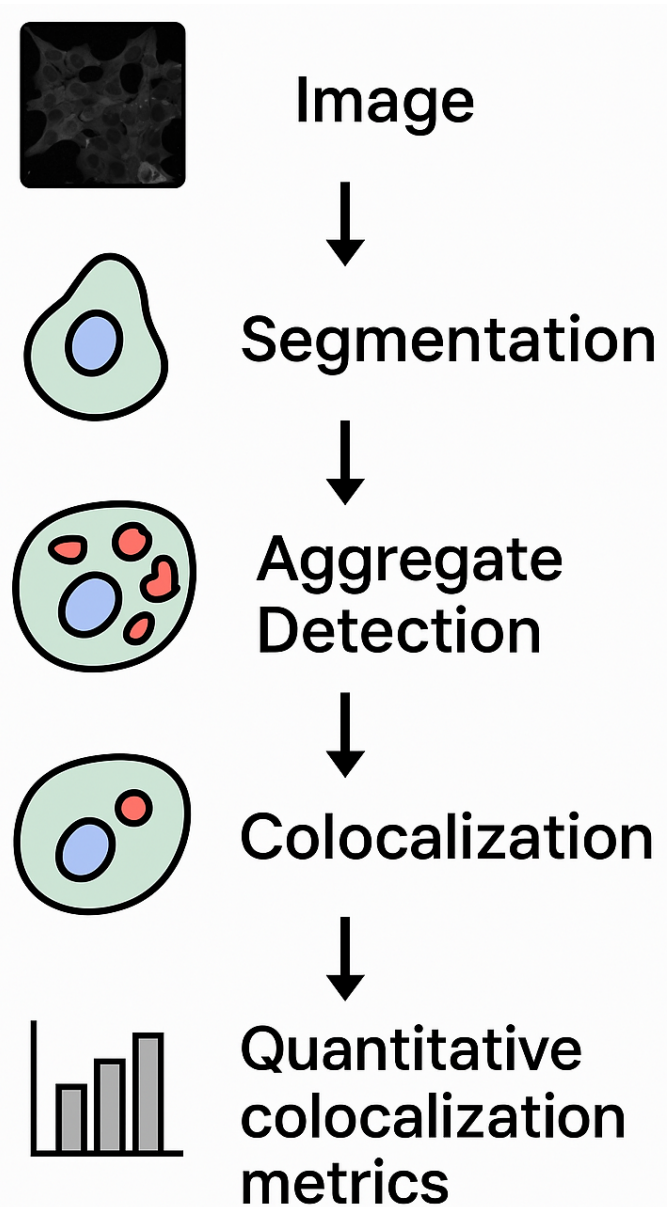
Fig. 3. Segmentation pipeline
