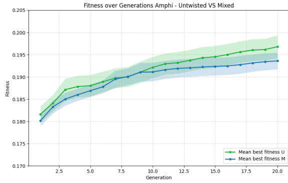
(b) Plot of the mixed (blue) and untwisted (green) populations on the amphitheater environment backward movement.
