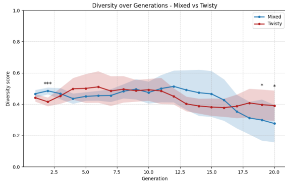
(b) Diversity scores of Mixed and Twisty populations for the flat terrain experiment with backward movement.
