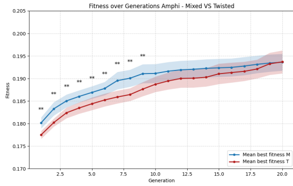
(a) Plot of the mixed (blue) and twisted (red) populations on the amphitheater environment for backward movement.
