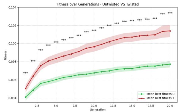
(c) Plot of the twisted (red) and untwisted (green) populations on the flat world environment for forward movement.
