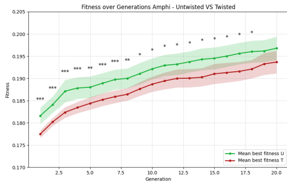
(c) Plot of the twisted (red) and untwisted (green) populations on the amphitheater environment backward movement.
