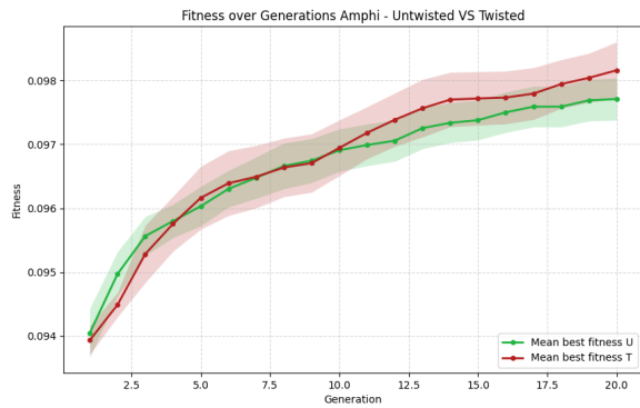
(c) Plot of the twisted (red) and untwisted (green) populations on the amphitheater environment forward movement.
