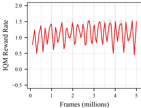
PPO (RTU only)
