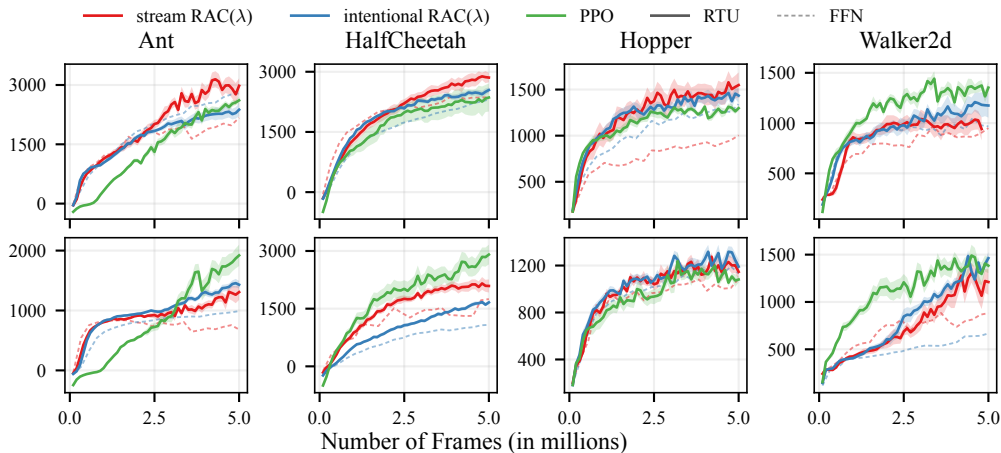
IQM Episode Return
