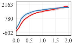
HalfCheetah
