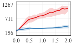
Walker2d
