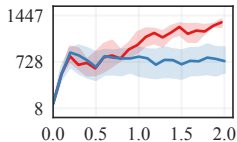
Hopper
