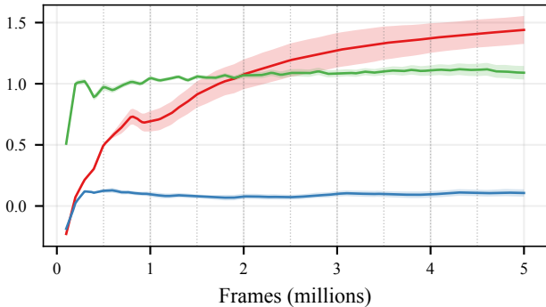
Average Reward
