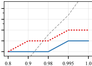
stream Q(\lambda)
