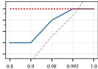
intentional Q(\lambda)
