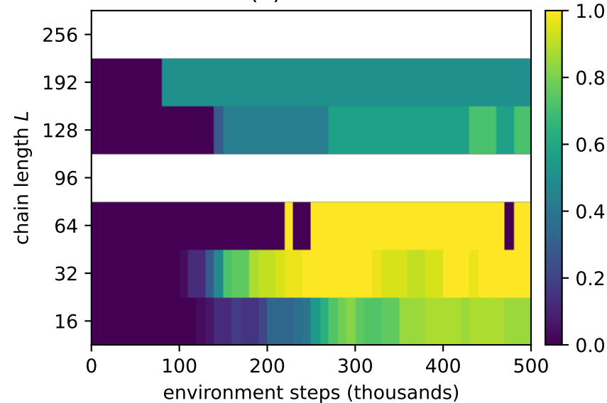
TBPTT(1): seeds solved
