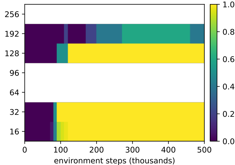
RTRL: seeds solved
