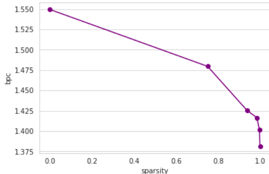
Figure 4: BPC vs Sparsity for Constant Parameter Count. Shows the same results as Table 2. The biggest, sparsest GRU performs better than a dense network with 6.25x as many (nonzero) parameters.
