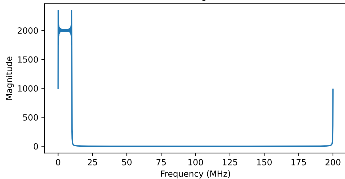
FFT of Signal B
