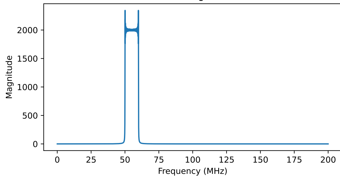
FFT of Signal C
