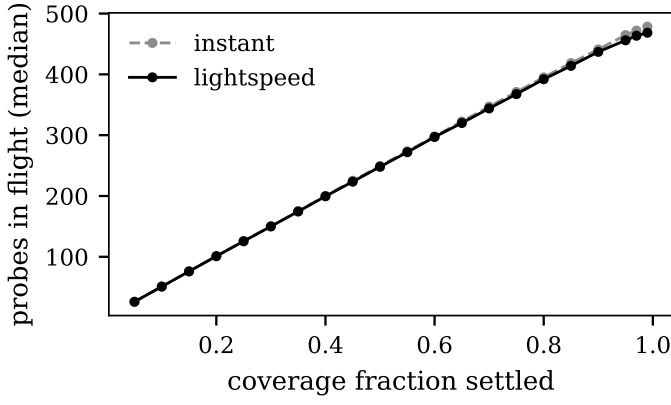
Fig. 2. Probes in flight versus the fraction of the field settled, for perfect information and the light-speed gate (medians over 16 seeds, 500-star field, \Lambda = 0.2 ). The population stays near its peak of a few hundred all the way into the final percent and the two regimes track each other closely, so the fills run almost in lockstep and the light-lag swarm loses only the small productive-rate deficit that keeps the time tax a fraction of the fuel tax.
