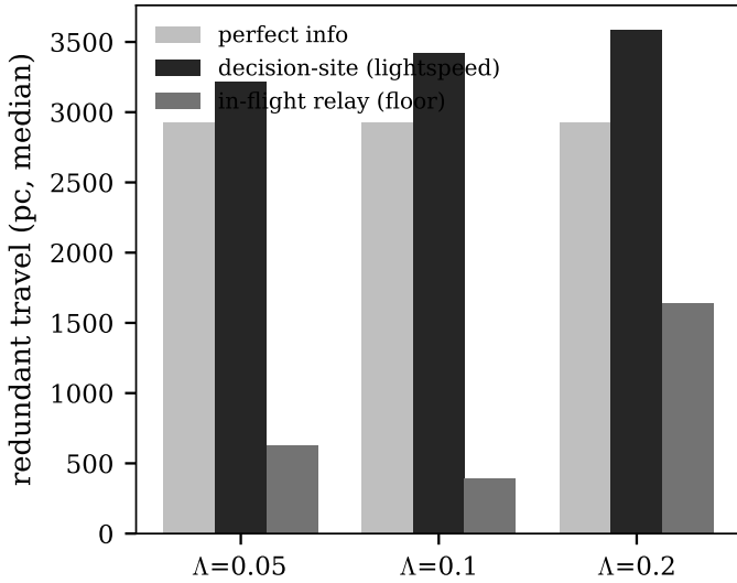
Fig. 6. Redundant travel under perfect information, the decision-site light-speed gate, and in-flight relay, versus \Lambda (medians over 48 seeds, 400-star field). Listening in flight drives completed wasted arrivals to zero and cuts redundant travel below even the perfect-information baseline, recovering the light-lag tax at a small cost in fill time.
