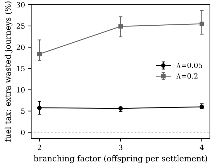
Fig. 5. Fuel tax versus the replication branching factor (offspring per settlement) at moderate and directed-energy speed, over the 32-seed ensemble (points: medians; bars: bootstrap 95% confidence intervals). Contention grows with branching at high \Lambda and then saturates; the default of two offspring does not hide a much larger tax.
