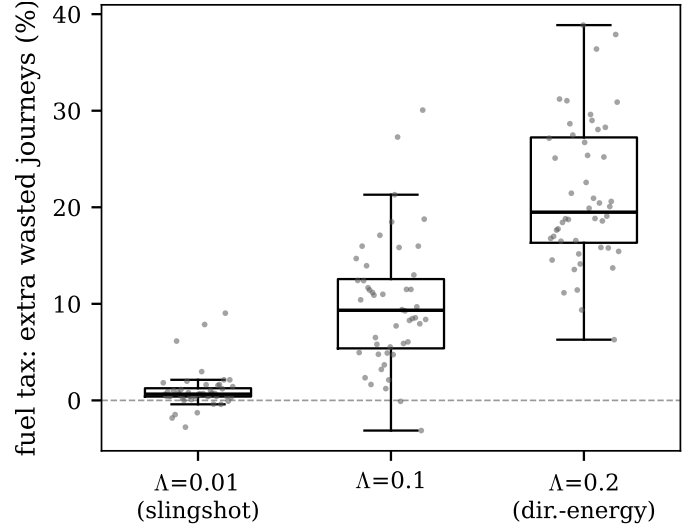
Fig. 4. Per-seed distribution of the fuel tax (extra wasted journeys, as a percent of the perfect-information waste) at slingshot speed ( \Lambda = 0.01 ), \Lambda = 0.1 , and directed-energy speed ( \Lambda = 0.2 ), over the 48-seed ensemble (box: interquartile range and median; points: individual seeds). The tax is small but consistently positive at slingshot speed and unambiguous at directed-energy speed.
