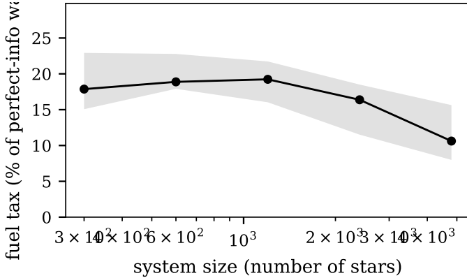
Fig. 7. Fuel tax as a percent of the perfect-information waste versus system size, at \Lambda = 0.2 (point: median; shaded band: bootstrap 95% confidence interval). Over a sixteen-fold range the tax holds near 18 to 19% up to about a thousand stars and then trends downward at the largest, fewest-seed fields; it does not grow with scale, so nothing here supports extrapolating a fixed-percentage tax to galactic size.
