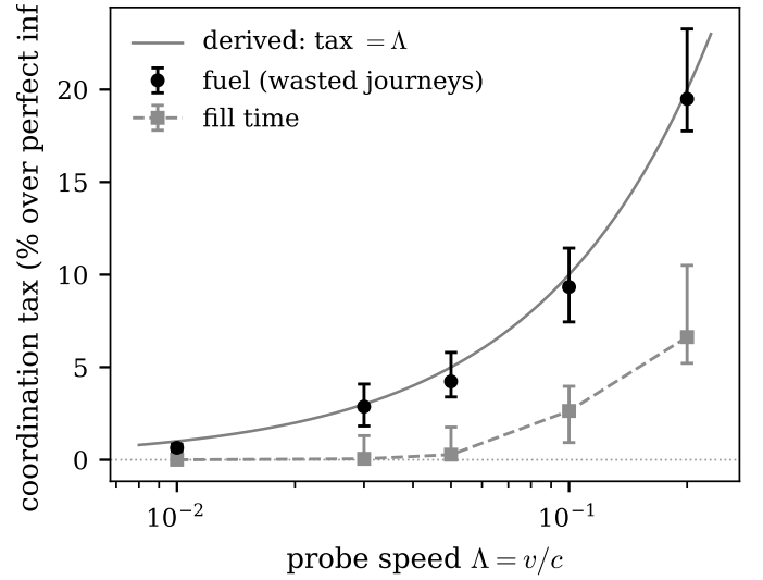
Fig. 3. The coordination tax versus probe speed \Lambda = v/c , powered flight, over the 48-seed ensemble at the event-driven timestep (points: medians; bars: bootstrap 95% confidence intervals). The redundant-travel (fuel) tax sits on the derived law tax = \Lambda (grey line, Eq. 3) at every speed; the fill-time tax stays near zero at slingshot speeds and emerges to a few percent only in the directed-energy regime.
