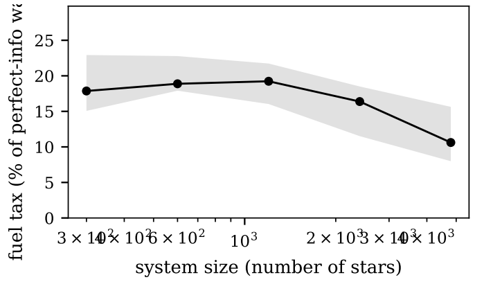
Fig. 7. Fuel tax as a percent of the perfect-information waste versus system size, at \Lambda = 0.2 (point: median; shaded band: bootstrap 95% confidence interval). Over a sixteen-fold range the tax holds near 18 to 19% up to about a thousand stars and then trends downward at the largest, fewest-seed fields; it does not grow with scale, so nothing here supports extrapolating a fixed-percentage tax to galactic size.
