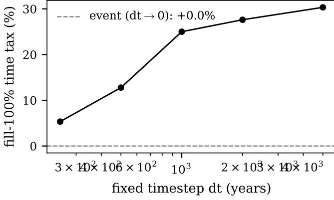
Fig. 1. The fill-100% time penalty for nearest-star slingshot flight versus the fixed timestep, over the 32-seed ensemble. The apparent penalty is monotone in the step and collapses to zero (dashed line: the event-driven, dt-independent limit). The tens-of-percent “coordination tax” of a coarse-step model is a discretization artifact, not a physical slowdown.
