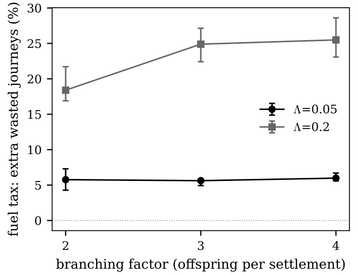
Fig. 6. Fuel tax versus the replication branching factor (offspring per settlement) at moderate and directed-energy speed, over the 32-seed ensemble (points: medians; bars: bootstrap 95% confidence intervals). Contention grows with branching at high \Lambda and then saturates; the default of two offspring does not hide a much larger tax.
