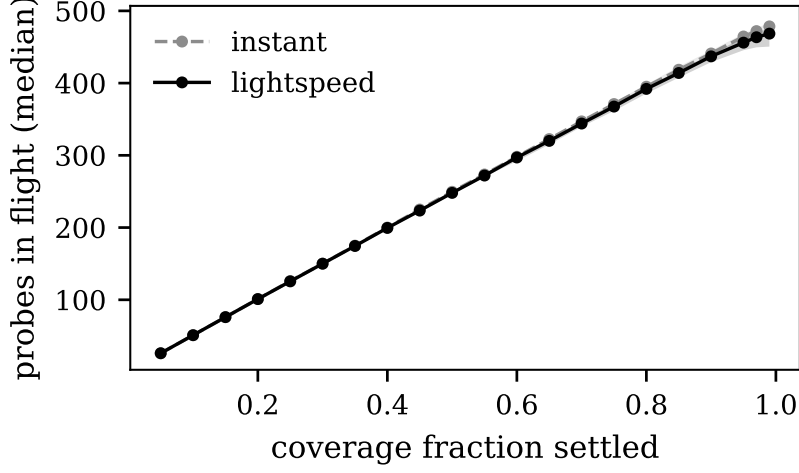
Figure 2: Probes in flight versus the fraction of the field settled, for perfect information and the light-speed gate (medians over 16 seeds with bootstrap 95% confidence bands, 500-star field, \Lambda = 0.2 ). The population stays near its peak of a few hundred all the way into the final percent and the two regimes track each other closely, so the fills run almost in lockstep and the light-lag swarm loses only the small productive-rate deficit that keeps the time tax a fraction of the fuel tax.
