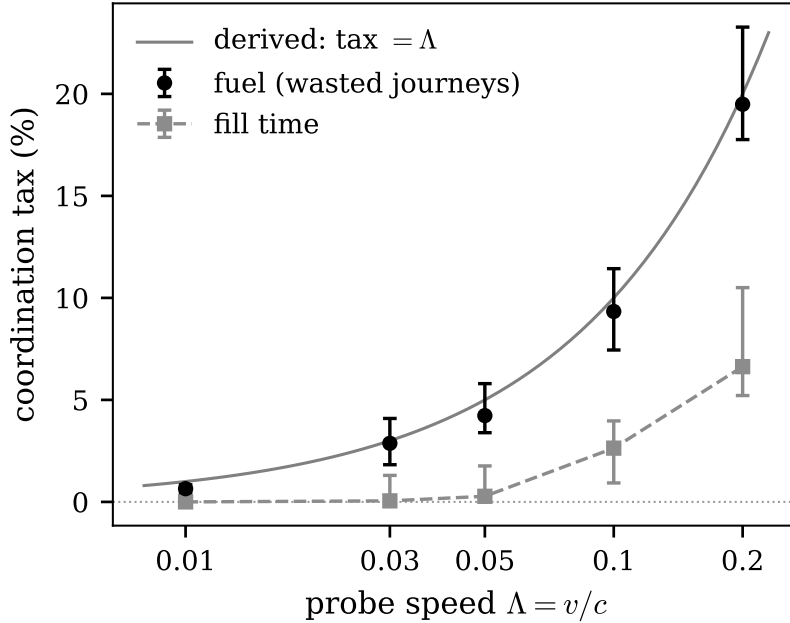
Figure 3: The coordination tax versus probe speed \Lambda = v/c (log axis, so the linear law tax = \Lambda appears as an upward curve), powered flight, over the 48-seed ensemble at the event-driven timestep (both as a percent over perfect information; points: medians; bars: bootstrap 95% confidence intervals). The redundant-travel (fuel) tax sits on the derived law tax = \Lambda (grey line, Eq. 3) at every speed; the fill-time tax stays near zero at slingshot speeds and emerges to a few percent only in the directed-energy regime.
